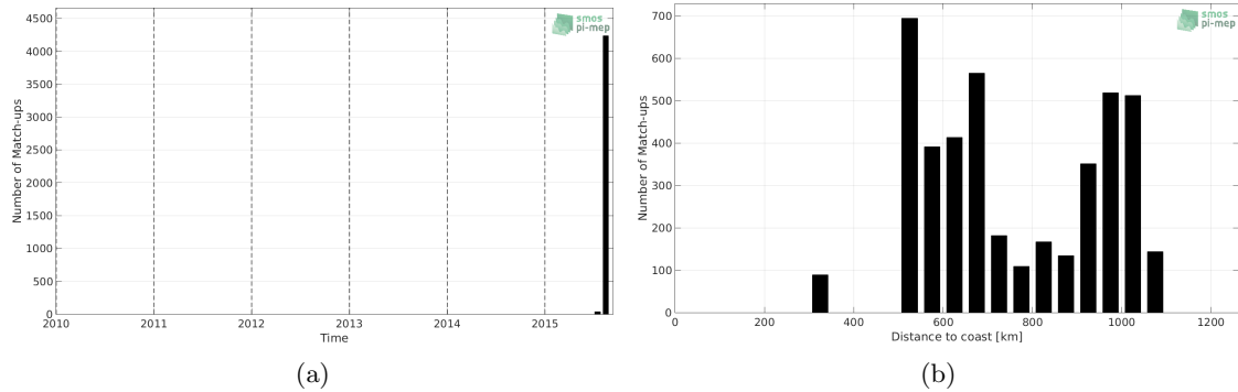
Figure 1: Number of match-ups between TSG-GOSUD-Research-vessel and SMAP-L3-RSS-V4-8DAY-RUNNING SSS as a function of time (a) and as function of the distance to coast (b) over the North Pacific Ocean Pi-MEP region and for the full satellite product period.
