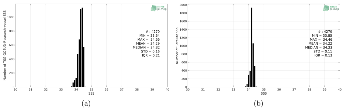
Figure 2: Histograms of SSS from TSG-GOSUD-Research-vessel (a) and SMAP-L3-RSS-V4-8DAY-RUNNING (b) considering all match-up pairs per bins of 0.1 over the North Pacific Ocean Pi-MEP region and for the full satellite product period.
