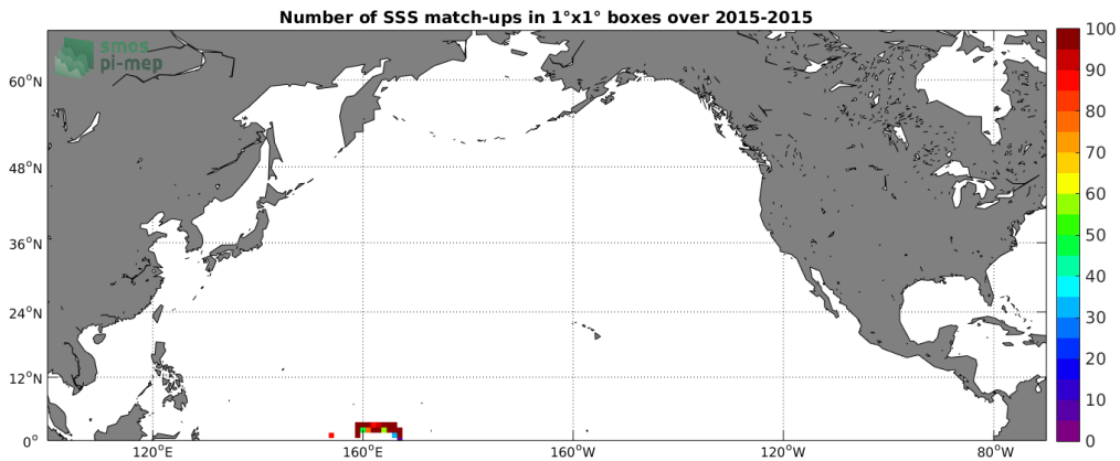
Figure 4: Number of SSS match-ups between TSG-GOSUD-Research-vessel SSS and the SMAP-L3-RSS-V4-8DAY-RUNNING SSS product for the North Pacific Ocean Pi-MEP region over 1°x1° boxes and for the full satellite product period.
