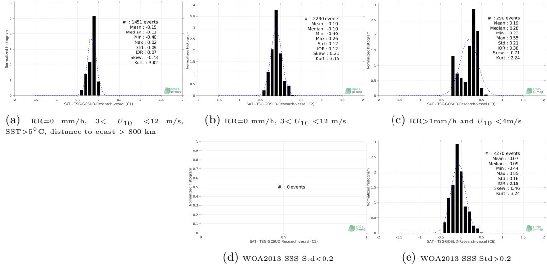
Figure 13: Normalized histogram of \Delta\text{SSS} (SMAP-L3-RSS-V4-8DAY-RUNNING - TSG-GOSUD-Research-vessel) for 5 different subdatasets corresponding to: RR=0 mm/h, 3 < U_{10} < 12 m/s, SST > 5^{\circ}\text{C} , distance to coast > 800 km (a), RR=0 mm/h, 3 < U_{10} < 12 m/s (b), RR > 1\text{mm/h} and U_{10} < 4\text{m/s} (c), WOA2013 SSS Std < 0.2 (d), WOA2013 SSS Std > 0.2 (e).
