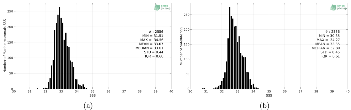
Figure 2: Histograms of SSS from Marine mammals (a) and SMAP SSS L3 v4 - 8-Day running (RSS) (b) considering all match-up pairs per bins of 0.1 over the North Pacific Ocean Pi-MEP region and for the full satellite product period.
