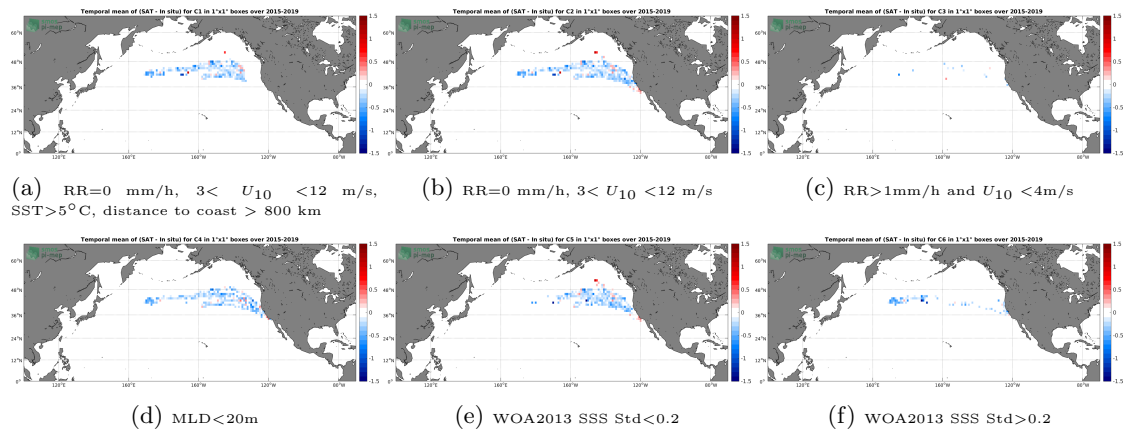
Figure 12: Temporal mean gridded over spatial boxes of size 1^\circ \times 1^\circ of \Delta SSS (SMAP SSS L3 v4 - 8-Day running (RSS) - Marine mammals) for 6 different subdatasets corresponding to:RR=0 mm/h, 3 < U_{10} < 12 m/s, SST >5^\circ\text{C} , distance to coast > 800 km (a), RR=0 mm/h, 3 < U_{10} < 12 m/s (b), RR >1 mm/h and U_{10} < 4 m/s (c),MLD <20 m (d),WOA2013 SSS Std <0.2 (e),WOA2013 SSS Std >0.2 (f).
