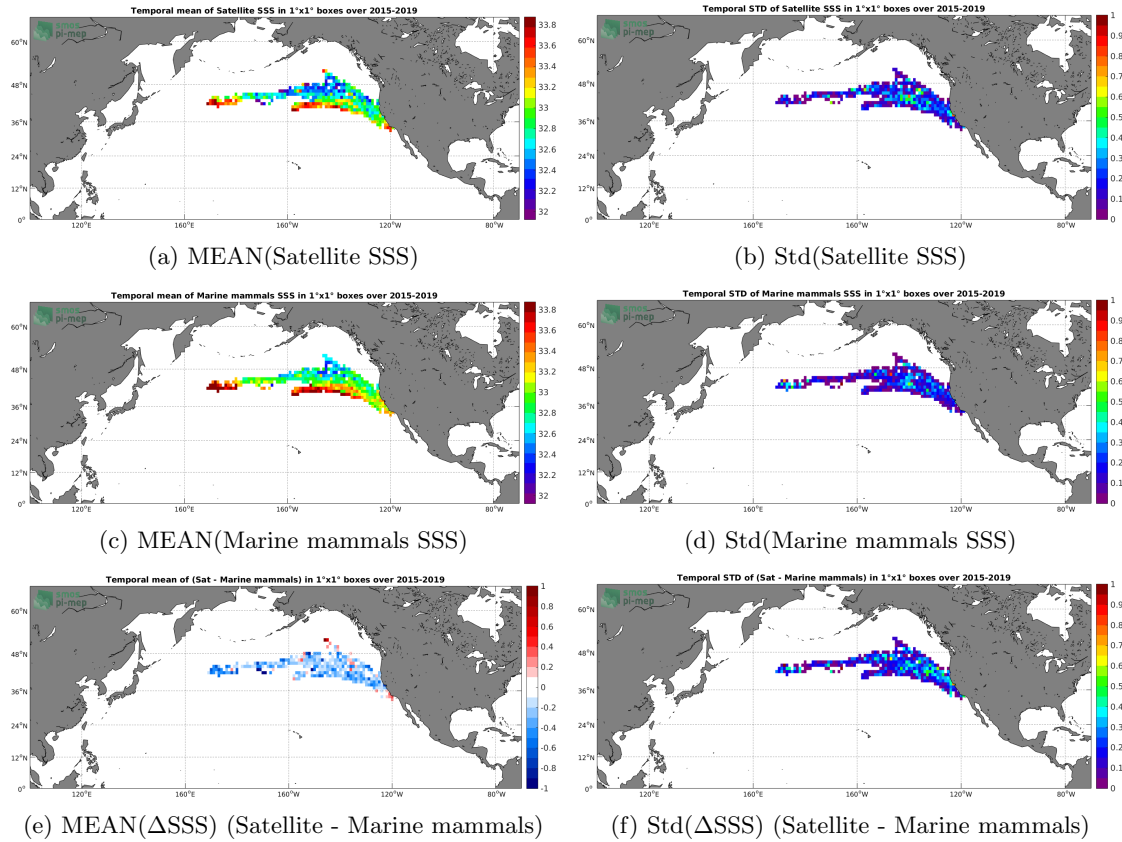
Figure 6: Temporal mean (left) and Std (right) of SSS from SMAP SSS L3 v4 - 8-Day running (RSS) (top), Marine mammals (middle), and of \Delta SSS (Satellite - Marine mammals). Only match-up pairs are used to generate these maps.
