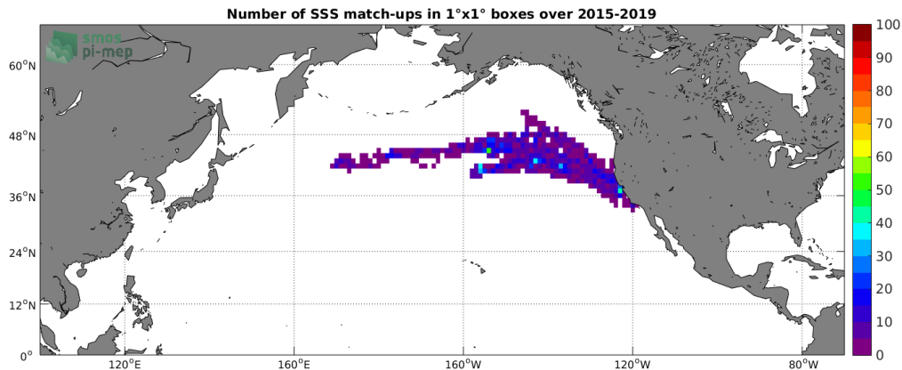
Figure 4: Number of SSS match-ups between Marine mammals SSS and the SMAP SSS L3 v4 - 8-Day running (RSS) SSS product for the North Pacific Ocean Pi-MEP region over 1^\circ \times 1^\circ boxes and for the full satellite product period.
