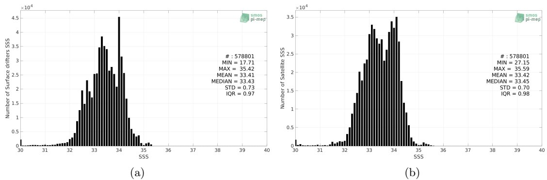
Figure 2: Histograms of SSS from Surface drifters (a) and SMAP SSS L3 v4 - 8-Day running (RSS) (b) considering all match-up pairs per bins of 0.1 over the North Pacific Ocean Pi-MEP region and for the full satellite product period.
