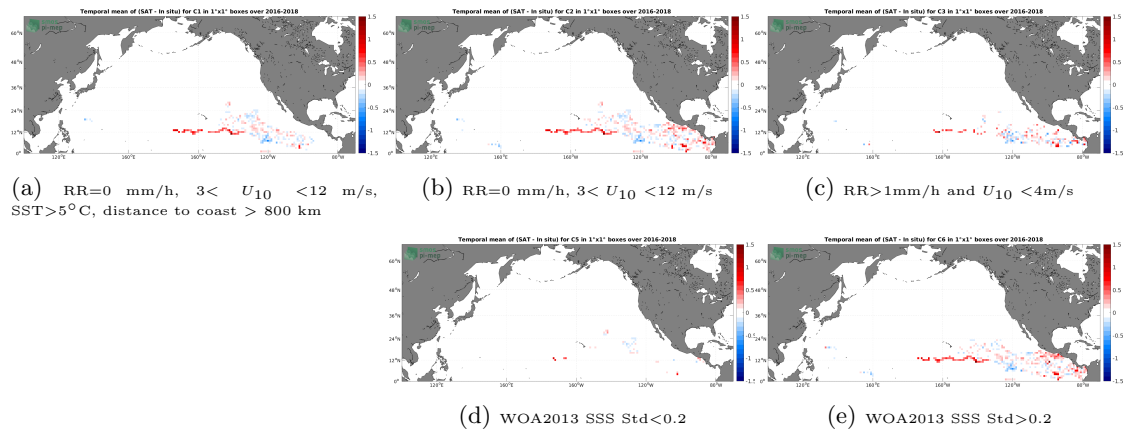
Figure 11: Temporal mean gridded over spatial boxes of size 1^\circ \times 1^\circ of \Delta SSS (SMAP SSS L3 v4 - 8-Day running (RSS) - Surface drifters) for 5 different subdatasets corresponding to:RR=0 mm/h, 3 < U_{10} < 12 m/s, SST >5^\circ C, distance to coast > 800 km (a), RR=0 mm/h, 3 < U_{10} < 12 m/s (b), RR >1 mm/h and U_{10} < 4 m/s (c), WOA2013 SSS Std <0.2 (d), WOA2013 SSS Std >0.2 (e).
