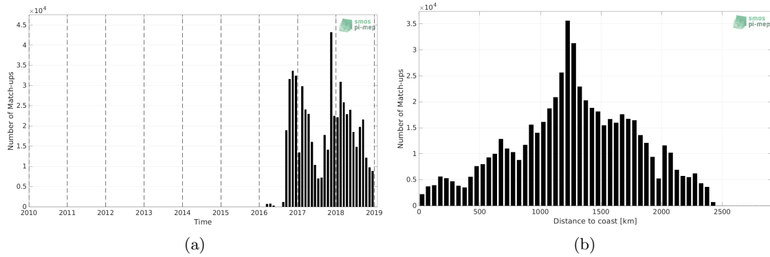
Figure 1: Number of match-ups between Surface drifters and SMAP SSS L3 v4 - 8-Day running (RSS) SSS as a function of time (a) and as function of the distance to coast (b) over the North Pacific Ocean Pi-MEP region and for the full satellite product period.
