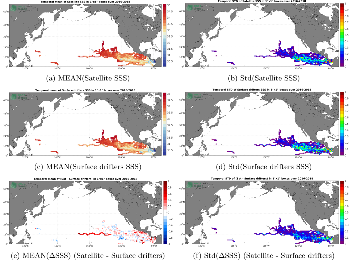
Figure 5: Temporal mean (left) and Std (right) of SSS from SMAP SSS L3 v4 - 8-Day running (RSS) (top), Surface drifters (middle), and of \Delta SSS (Satellite - Surface drifters). Only match-up pairs are used to generate these maps.
