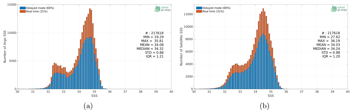
Figure 2: Histograms of SSS from Argo (a) and SMAP SSS L3 v4 - 8-Day running (RSS) (b) considering all match-up pairs per bins of 0.1 over the North Pacific Ocean Pi-MEP region and for the full satellite product period.
