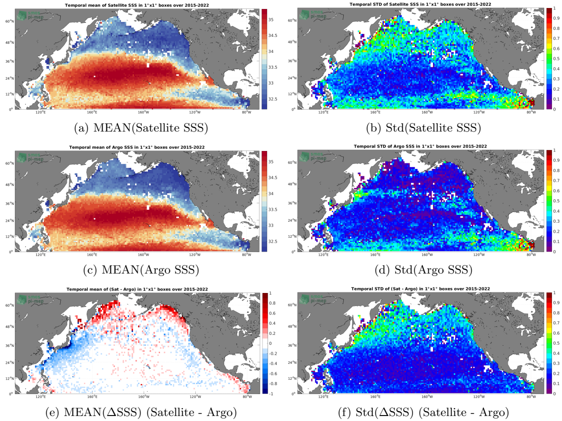
Figure 6: Temporal mean (left) and Std (right) of SSS from SMAP SSS L3 v4 - 8-Day running (RSS) (top), Argo (middle), and of \Delta SSS (Satellite - Argo). Only match-up pairs are used to generate these maps.
