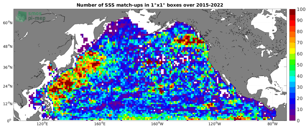
Figure 4: Number of SSS match-ups between Argo SSS and the SMAP SSS L3 v4 - 8-Day running (RSS) SSS product for the North Pacific Ocean Pi-MEP region over 1^\circ \times 1^\circ boxes and for the full satellite product period.
