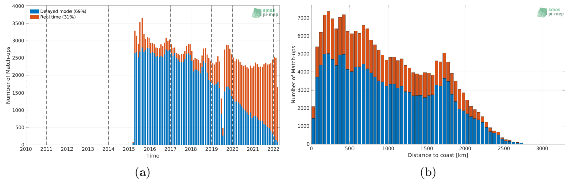
Figure 1: Number of match-ups between Argo and SMAP SSS L3 v4 - 8-Day running (RSS) SSS as a function of time (a) and as function of the distance to coast (b) over the North Pacific Ocean Pi-MEP region and for the full satellite product period.
