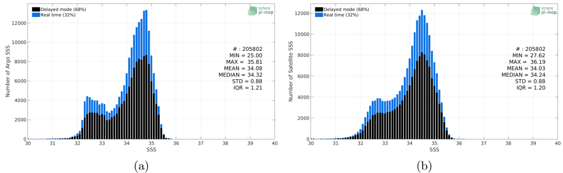
Figure 2: Histograms of SSS from Argo (a) and SMAP SSS L3 v4 - 8-Day running (RSS) (b) considering all match-up pairs per bins of 0.1 over the North Pacific Ocean Pi-MEP region and for the full satellite product period.
