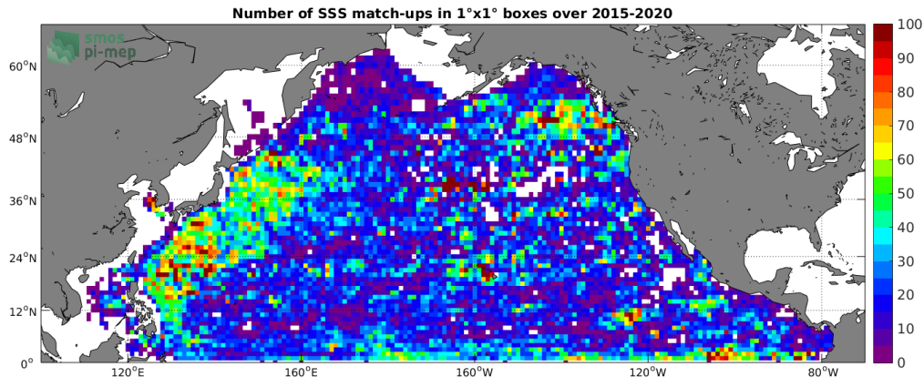
Figure 4: Number of SSS match-ups between Argo SSS and the SMAP-L3-RSS-V4-8DAY-RUNNING SSS product for the North Pacific Ocean Pi-MEP region over 1^\circ \times 1^\circ boxes and for the full satellite product period.
