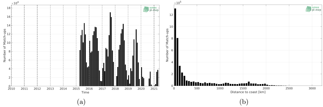
Figure 1: Number of match-ups between TSG (SAMOS) and SMAP SSS L3 v4 - Monthly (RSS) SSS as a function of time (a) and as function of the distance to coast (b) over the North Pacific Ocean Pi-MEP region and for the full satellite product period.
