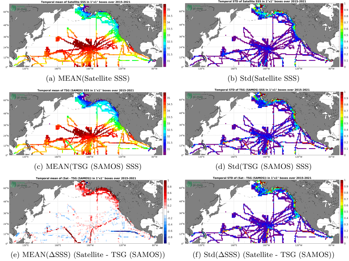
Figure 6: Temporal mean (left) and Std (right) of SSS from SMAP SSS L3 v4 - Monthly (RSS) (top), TSG (SAMOS) (middle), and of \Delta SSS (Satellite - TSG (SAMOS)). Only match-up pairs are used to generate these maps.
