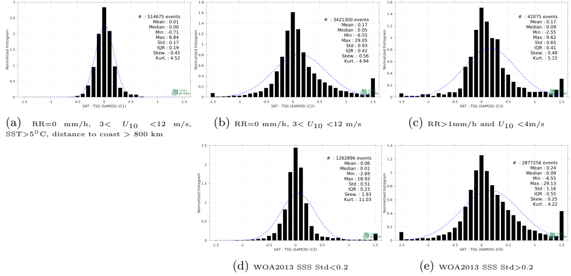
Figure 13: Normalized histogram of \Delta\text{SSS} (SMAP SSS L3 v4 - Monthly (RSS) - TSG (SAMOS)) for 5 different subdatasets corresponding to: RR=0 mm/h, 3 < U_{10} < 12 m/s, SST>5°C, distance to coast > 800 km (a), RR=0 mm/h, 3 < U_{10} < 12 m/s (b), RR>1mm/h and U_{10} < 4 m/s (c), WOA2013 SSS Std<0.2 (d), WOA2013 SSS Std>0.2 (e).
