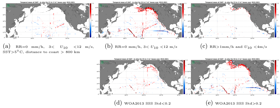
Figure 12: Temporal mean gridded over spatial boxes of size 1^\circ \times 1^\circ of \Delta SSS (SMAP SSS L3 v4 - Monthly (RSS) - TSG (SAMOS)) for 5 different subdatasets corresponding to: RR=0 mm/h, 3 < U_{10} < 12 m/s, SST > 5^\circ C , distance to coast > 800 km (a), RR=0 mm/h, 3 < U_{10} < 12 m/s (b), RR > 1 mm/h and U_{10} < 4 m/s (c), WOA2013 SSS Std < 0.2 (d), WOA2013 SSS Std > 0.2 (e).
