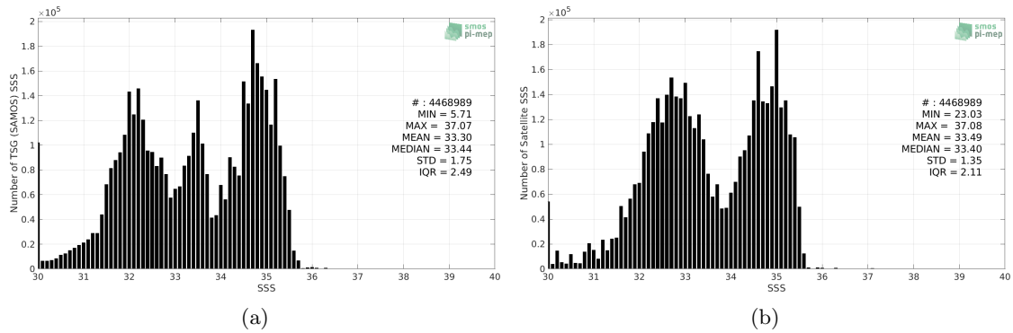
Figure 2: Histograms of SSS from TSG (SAMOS) (a) and SMAP SSS L3 v4 - Monthly (RSS) (b) considering all match-up pairs per bins of 0.1 over the North Pacific Ocean Pi-MEP region and for the full satellite product period.
