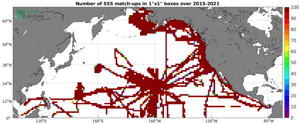
Figure 4: Number of SSS match-ups between TSG (SAMOS) SSS and the SMAP SSS L3 v4 - Monthly (RSS) SSS product for the North Pacific Ocean Pi-MEP region over 1^\circ \times 1^\circ boxes and for the full satellite product period.
