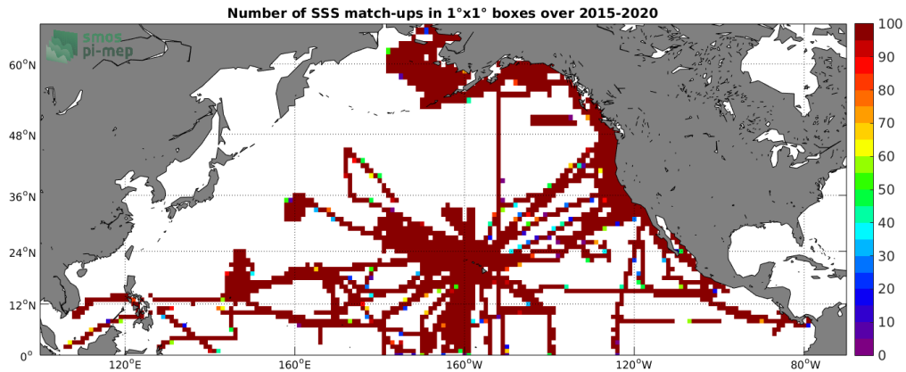
Figure 4: Number of SSS match-ups between TSG-SAMOS SSS and the SMAP-L3-RSS-V4-MONTHLY SSS product for the North Pacific Ocean Pi-MEP region over 1°x1° boxes and for the full satellite product period.
