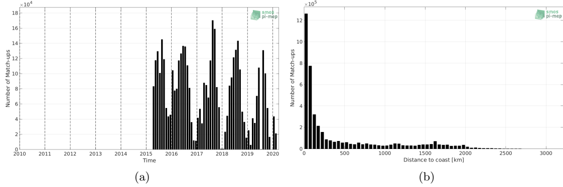
Figure 1: Number of match-ups between TSG-SAMOS and SMAP-L3-RSS-V4-MONTHLY SSS as a function of time (a) and as function of the distance to coast (b) over the North Pacific Ocean Pi-MEP region and for the full satellite product period.
