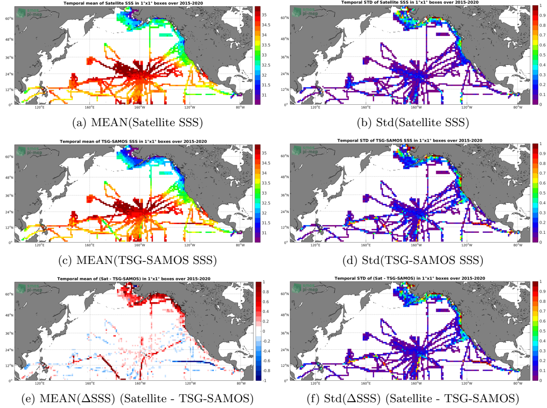
Figure 6: Temporal mean (left) and Std (right) of SSS from SMAP-L3-RSS-V4-MONTHLY (top), TSG-SAMOS (middle), and of \Delta SSS (Satellite - TSG-SAMOS). Only match-up pairs are used to generate these maps.
