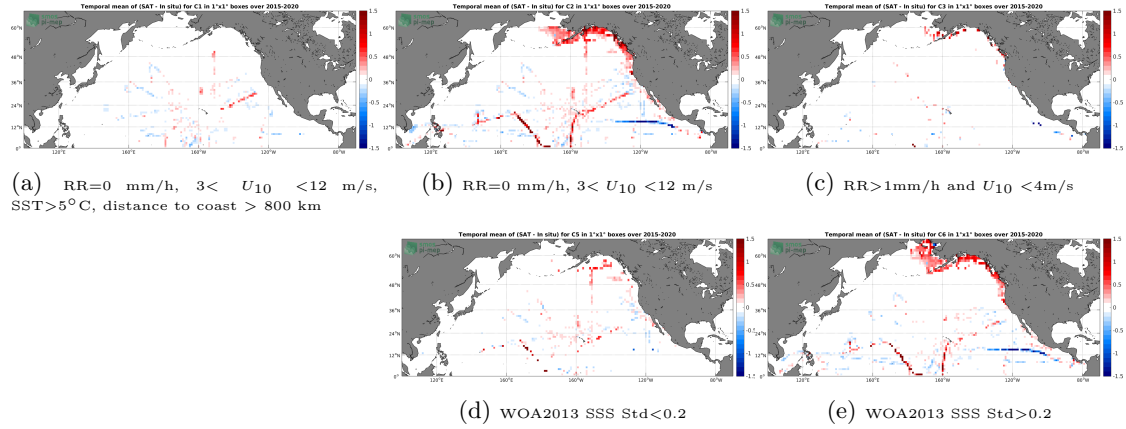
Figure 12: Temporal mean gridded over spatial boxes of size 1^\circ \times 1^\circ of \Delta SSS (SMAP-L3-RSS-V4-MONTHLY - TSG-SAMOS) for 5 different subdatasets corresponding to: RR=0 mm/h, 3 < U_{10} < 12 m/s, SST > 5^\circ C , distance to coast > 800 km (a), RR=0 mm/h, 3 < U_{10} < 12 m/s (b), RR > 1 mm/h and U_{10} < 4 m/s (c), WOA2013 SSS Std < 0.2 (d), WOA2013 SSS Std > 0.2 (e).
