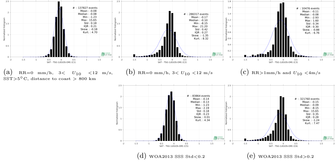
Figure 13: Normalized histogram of \Delta\text{SSS} (SMAP SSS L3 v4 - Monthly (RSS) - TSG (LEGOS-DM)) for 5 different subdatasets corresponding to: RR=0 mm/h, 3 < U_{10} < 12 m/s, SST>5°C, distance to coast > 800 km (a), RR=0 mm/h, 3 < U_{10} < 12 m/s (b), RR>1mm/h and U_{10} < 4 m/s (c), WOA2013 SSS Std<0.2 (d), WOA2013 SSS Std>0.2 (e).
