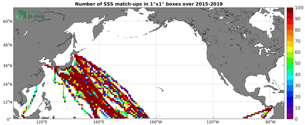
Figure 4: Number of SSS match-ups between TSG (LEGOS-DM) SSS and the SMAP SSS L3 v4 - Monthly (RSS) SSS product for the North Pacific Ocean Pi-MEP region over 1°x1° boxes and for the full satellite product period.
