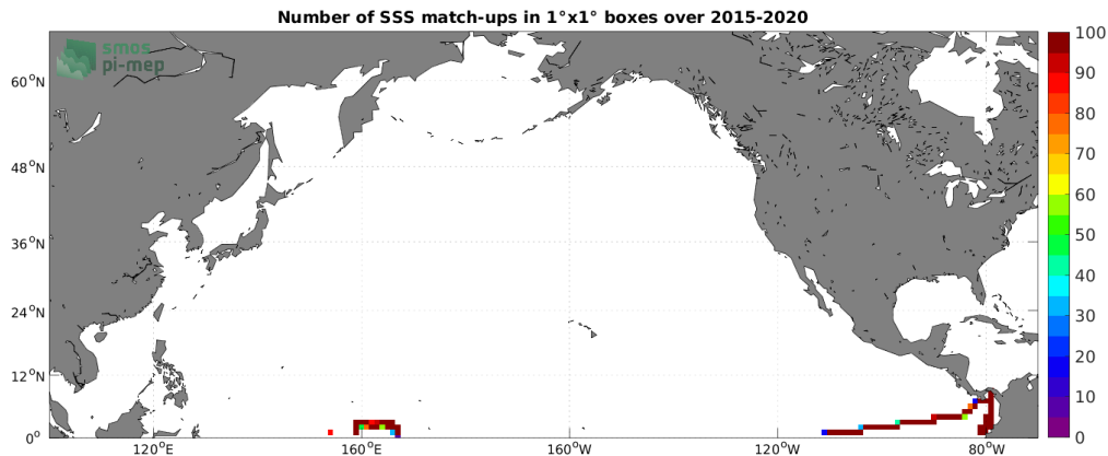
Figure 4: Number of SSS match-ups between TSG (GOSUD-Research-vessel) SSS and the SMAP SSS L3 v4 - Monthly (RSS) SSS product for the North Pacific Ocean Pi-MEP region over 1^\circ \times 1^\circ boxes and for the full satellite product period.
