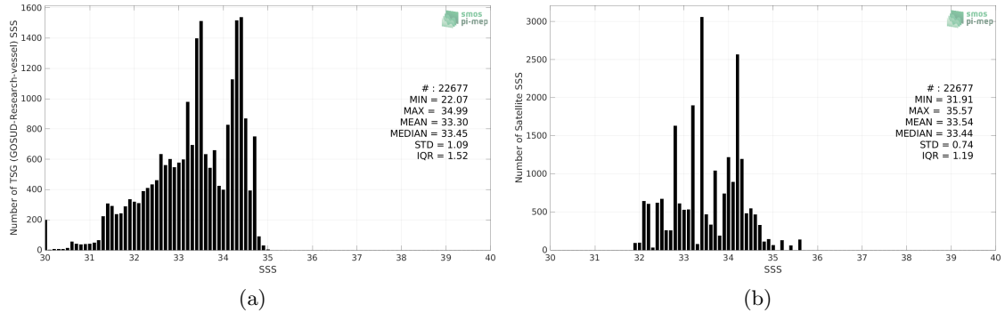
Figure 2: Histograms of SSS from TSG (GOSUD-Research-vessel) (a) and SMAP SSS L3 v4 - Monthly (RSS) (b) considering all match-up pairs per bins of 0.1 over the North Pacific Ocean Pi-MEP region and for the full satellite product period.
