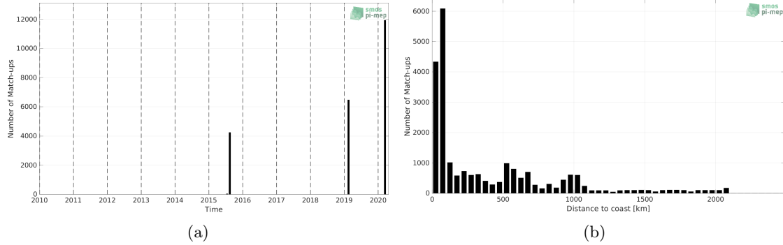
Figure 1: Number of match-ups between TSG (GOSUD-Research-vessel) and SMAP SSS L3 v4 - Monthly (RSS) SSS as a function of time (a) and as function of the distance to coast (b) over the North Pacific Ocean Pi-MEP region and for the full satellite product period.
