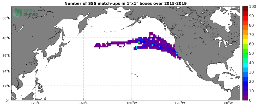
Figure 4: Number of SSS match-ups between Marine mammals SSS and the SMAP SSS L3 v4 - Monthly (RSS) SSS product for the North Pacific Ocean Pi-MEP region over 1^\circ \times 1^\circ boxes and for the full satellite product period.
