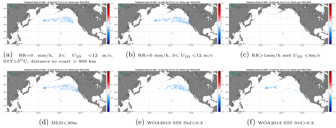
Figure 12: Temporal mean gridded over spatial boxes of size 1^\circ \times 1^\circ of \Delta SSS (SMAP SSS L3 v4 - Monthly (RSS) - Marine mammals) for 6 different subdatasets corresponding to: RR=0 mm/h, 3 < U_{10} < 12 m/s, SST > 5^\circ C , distance to coast > 800 km (a), RR=0 mm/h, 3 < U_{10} < 12 m/s (b), RR > 1 mm/h and U_{10} < 4 m/s (c), MLD < 20 m (d), WOA2013 SSS Std < 0.2 (e), WOA2013 SSS Std > 0.2 (f).
