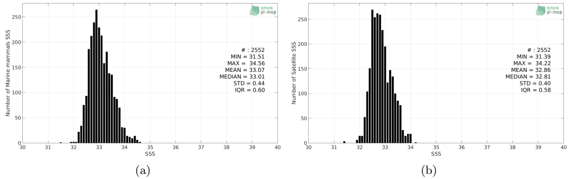
Figure 2: Histograms of SSS from Marine mammals (a) and SMAP SSS L3 v4 - Monthly (RSS) (b) considering all match-up pairs per bins of 0.1 over the North Pacific Ocean Pi-MEP region and for the full satellite product period.
