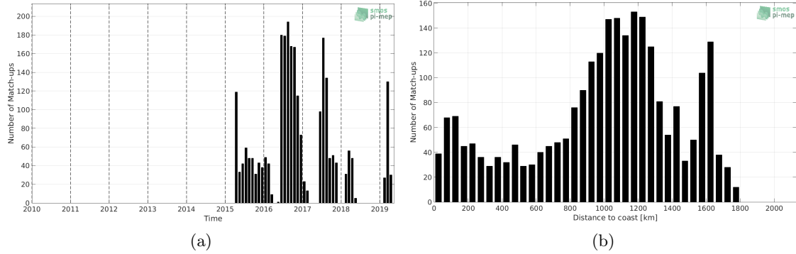
Figure 1: Number of match-ups between Marine mammals and SMAP SSS L3 v4 - Monthly (RSS) SSS as a function of time (a) and as function of the distance to coast (b) over the North Pacific Ocean Pi-MEP region and for the full satellite product period.
