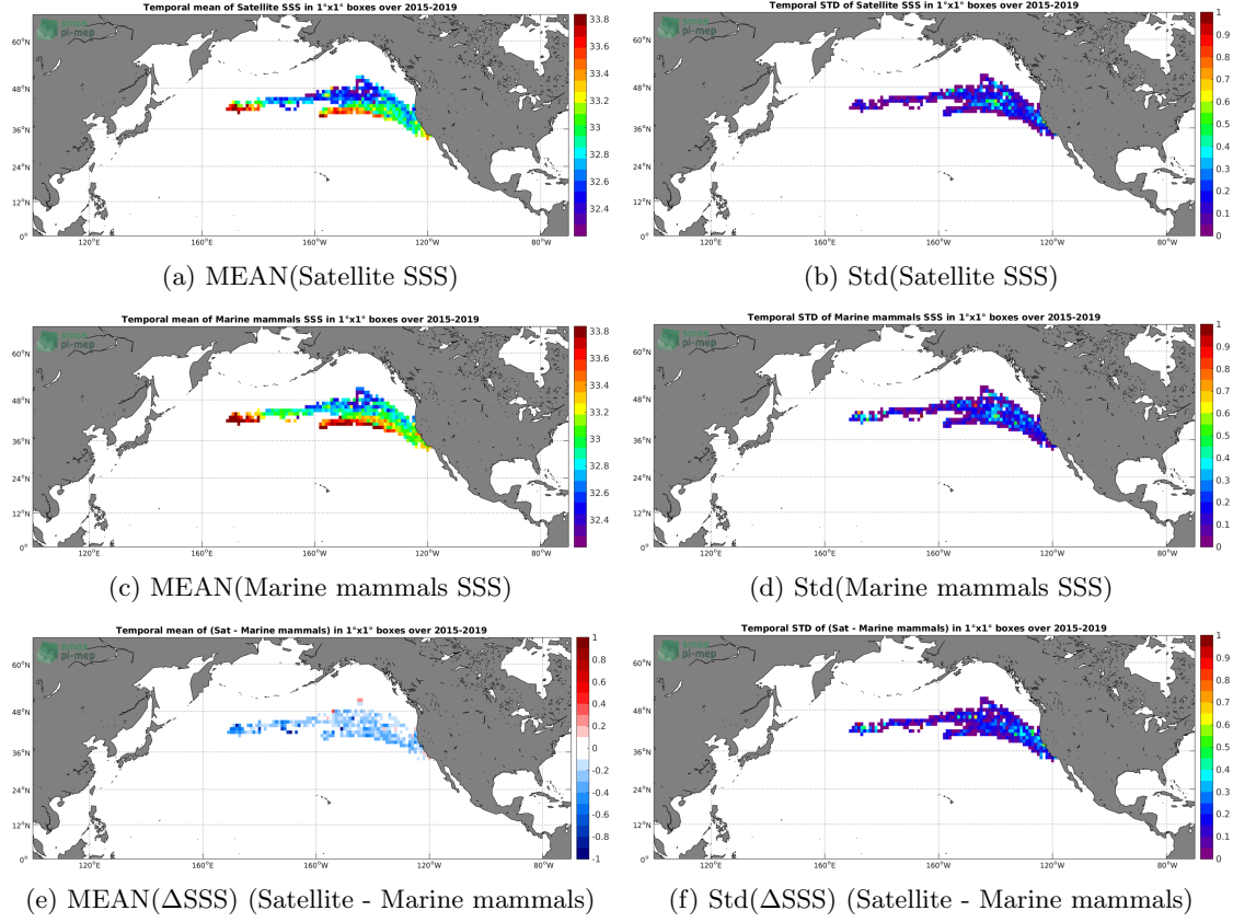
Figure 6: Temporal mean (left) and Std (right) of SSS from SMAP SSS L3 v4 - Monthly (RSS) (top), Marine mammals (middle), and of \Delta SSS (Satellite - Marine mammals). Only match-up pairs are used to generate these maps.
