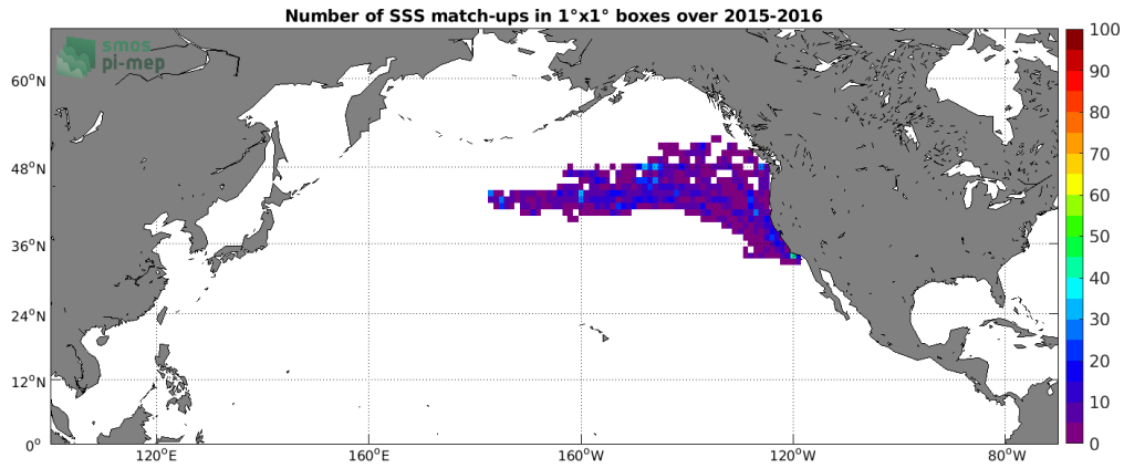
Figure 4: Number of SSS match-ups between Sea mammals SSS and the SMAP SSS L3 v4 - Monthly (RSS) SSS product for the North Pacific Ocean Pi-MEP region over 1^\circ \times 1^\circ boxes and for the full satellite product period.
