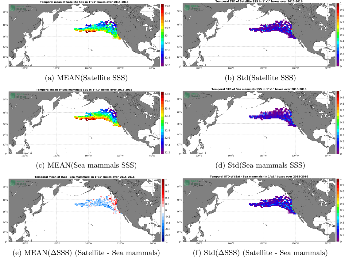
Figure 6: Temporal mean (left) and Std (right) of SSS from SMAP SSS L3 v4 - Monthly (RSS) (top), Sea mammals (middle), and of \Delta SSS (Satellite - Sea mammals). Only match-up pairs are used to generate these maps.
