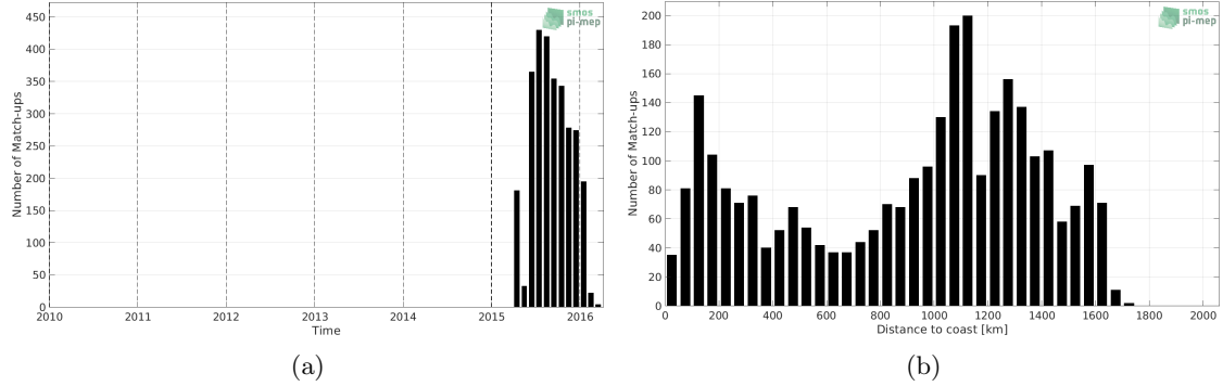
Figure 1: Number of match-ups between Sea mammals and SMAP SSS L3 v4 - Monthly (RSS) SSS as a function of time (a) and as function of the distance to coast (b) over the North Pacific Ocean Pi-MEP region and for the full satellite product period.
