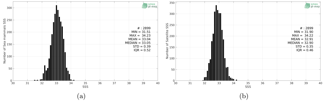
Figure 2: Histograms of SSS from Sea mammals (a) and SMAP SSS L3 v4 - Monthly (RSS) (b) considering all match-up pairs per bins of 0.1 over the North Pacific Ocean Pi-MEP region and for the full satellite product period.
