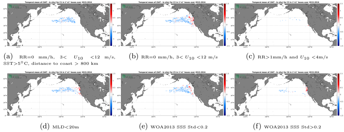
Figure 12: Temporal mean gridded over spatial boxes of size 1^\circ \times 1^\circ of \Delta SSS (SMAP SSS L3 v4 - Monthly (RSS) - Sea mammals) for 6 different subdatasets corresponding to: RR=0 mm/h, 3 < U_{10} < 12 m/s, SST > 5^\circ C , distance to coast > 800 km (a), RR=0 mm/h, 3 < U_{10} < 12 m/s (b), RR > 1 mm/h and U_{10} < 4 m/s (c), MLD < 20 m (d), WOA2013 SSS Std < 0.2 (e), WOA2013 SSS Std > 0.2 (f).
