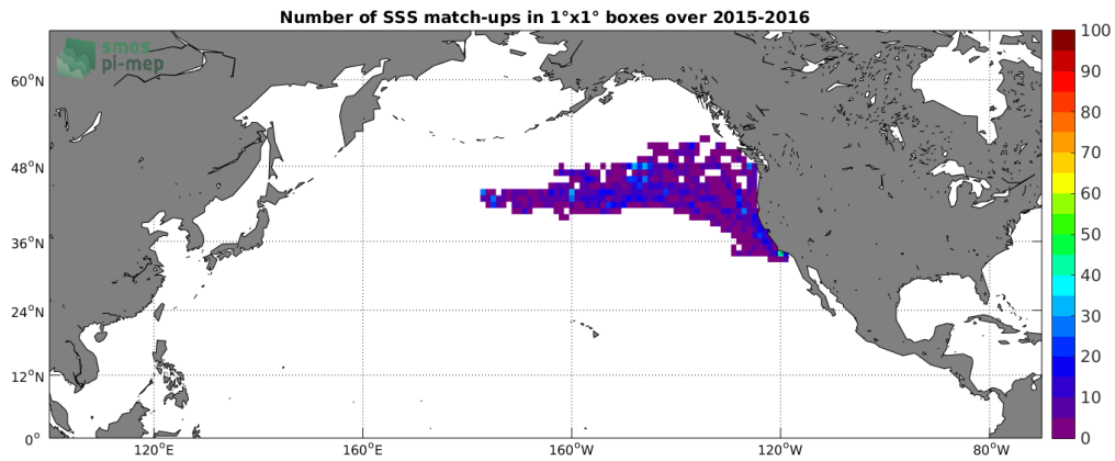
Figure 4: Number of SSS match-ups between Sea mammals SSS and the SMAP-L3-RSS-V4-MONTHLY SSS product for the North Pacific Ocean Pi-MEP region over 1°x1° boxes and for the full satellite product period.
