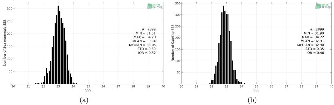
Figure 2: Histograms of SSS from Sea mammals (a) and SMAP-L3-RSS-V4-MONTHLY (b) considering all match-up pairs per bins of 0.1 over the North Pacific Ocean Pi-MEP region and for the full satellite product period.
