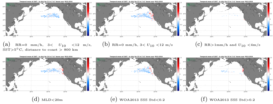
Figure 12: Temporal mean gridded over spatial boxes of size 1^\circ \times 1^\circ of \Delta SSS (SMAP-L3-RSS-V4-MONTHLY - Sea mammals) for 6 different subdatasets corresponding to: RR=0 mm/h, 3 < U_{10} < 12 m/s, SST > 5^\circ C , distance to coast > 800 km (a), RR=0 mm/h, 3 < U_{10} < 12 m/s (b), RR > 1 mm/h and U_{10} < 4 m/s (c), MLD < 20 m (d), WOA2013 SSS Std < 0.2 (e), WOA2013 SSS Std > 0.2 (f).
