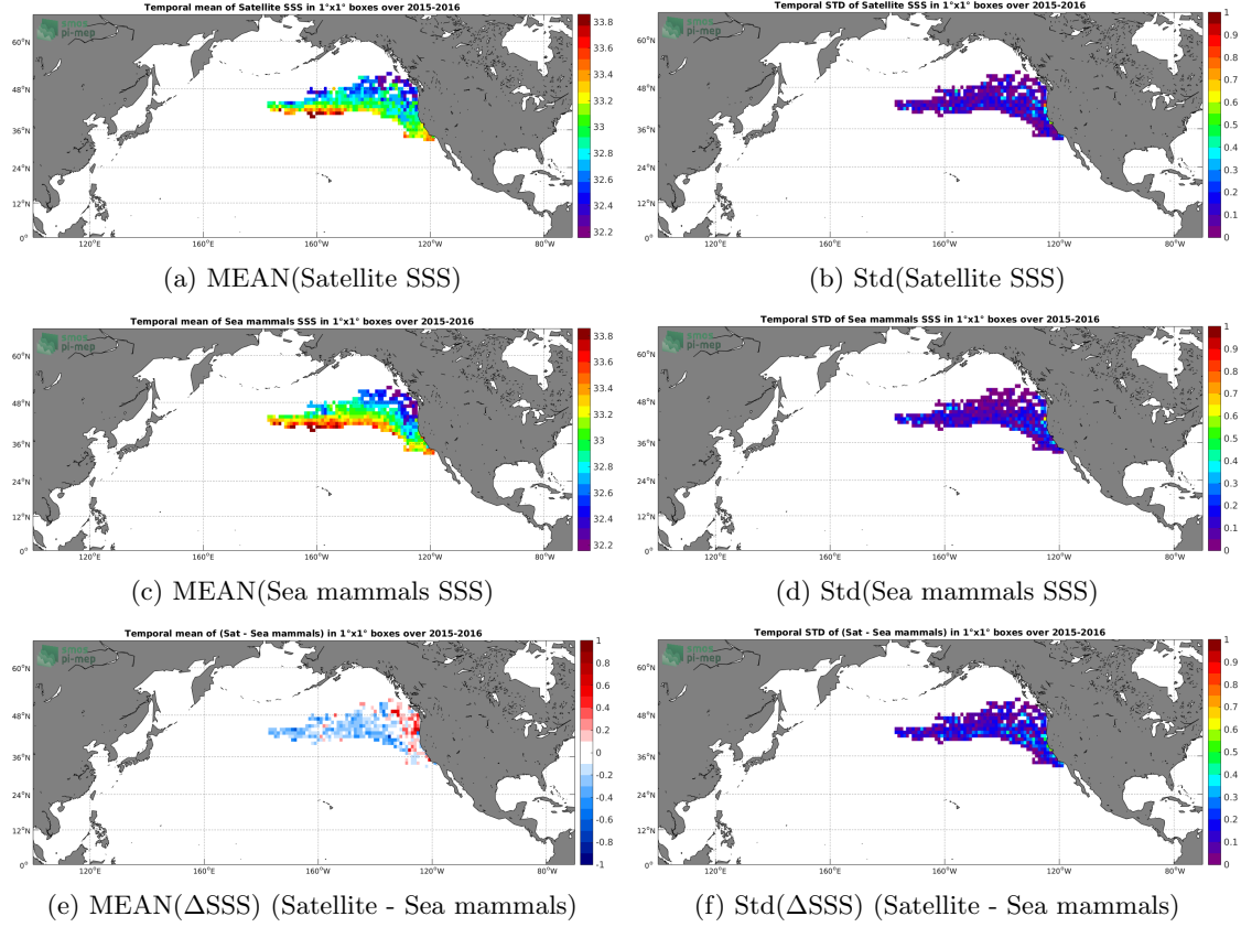
Figure 6: Temporal mean (left) and Std (right) of SSS from SMAP-L3-RSS-V4-MONTHLY (top), Sea mammals (middle), and of \Delta SSS (Satellite - Sea mammals). Only match-up pairs are used to generate these maps.
