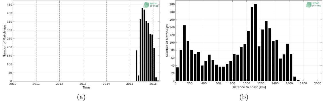
Figure 1: Number of match-ups between Sea mammals and SMAP-L3-RSS-V4-MONTHLY SSS as a function of time (a) and as function of the distance to coast (b) over the North Pacific Ocean Pi-MEP region and for the full satellite product period.
