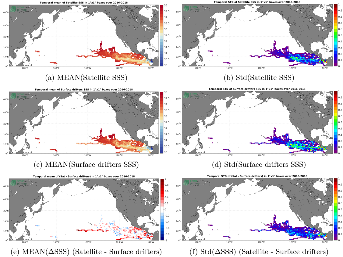
Figure 5: Temporal mean (left) and Std (right) of SSS from SMAP SSS L3 v4 - Monthly (RSS) (top), Surface drifters (middle), and of \Delta SSS (Satellite - Surface drifters). Only match-up pairs are used to generate these maps.
