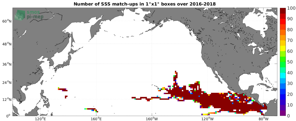
Figure 3: Number of SSS match-ups between Surface drifters SSS and the SMAP SSS L3 v4 - Monthly (RSS) SSS product for the North Pacific Ocean Pi-MEP region over 1^\circ \times 1^\circ boxes and for the full satellite product period.
