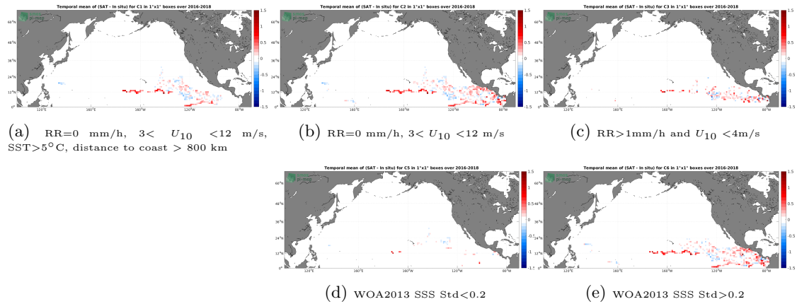
Figure 11: Temporal mean gridded over spatial boxes of size 1^\circ \times 1^\circ of \Delta SSS (SMAP SSS L3 v4 - Monthly (RSS) - Surface drifters) for 5 different subdatasets corresponding to:RR=0 mm/h, 3 < U_{10} < 12 m/s, SST > 5^\circ C , distance to coast > 800 km (a), RR=0 mm/h, 3 < U_{10} < 12 m/s (b), RR >1 mm/h and U_{10} < 4 m/s (c), WOA2013 SSS Std <0.2 (d), WOA2013 SSS Std >0.2 (e).
