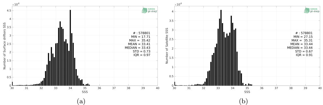
Figure 2: Histograms of SSS from Surface drifters (a) and SMAP SSS L3 v4 - Monthly (RSS) (b) considering all match-up pairs per bins of 0.1 over the North Pacific Ocean Pi-MEP region and for the full satellite product period.
