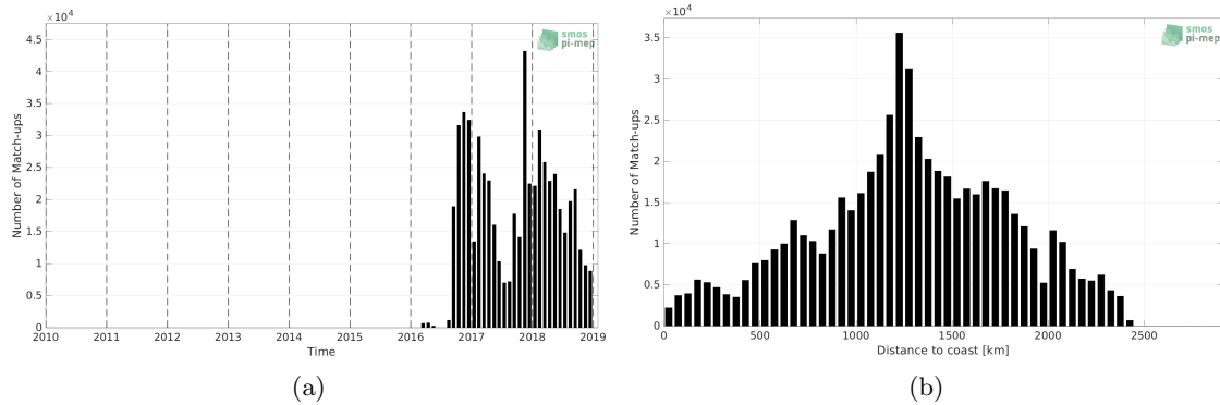
Figure 1: Number of match-ups between Surface drifters and SMAP SSS L3 v4 - Monthly (RSS) SSS as a function of time (a) and as function of the distance to coast (b) over the North Pacific Ocean Pi-MEP region and for the full satellite product period.
