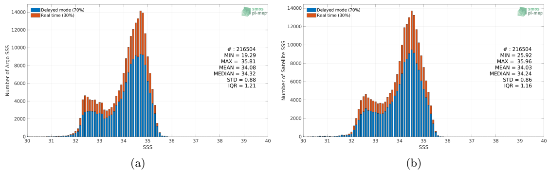
Figure 2: Histograms of SSS from Argo (a) and SMAP SSS L3 v4 - Monthly (RSS) (b) considering all match-up pairs per bins of 0.1 over the North Pacific Ocean Pi-MEP region and for the full satellite product period.
