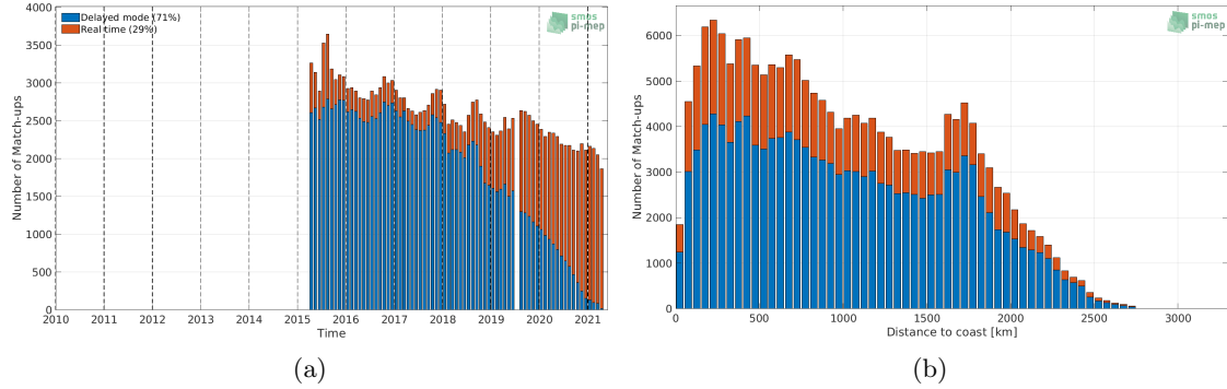
Figure 1: Number of match-ups between Argo and SMAP SSS L3 v4 - Monthly (RSS) SSS as a function of time (a) and as function of the distance to coast (b) over the North Pacific Ocean Pi-MEP region and for the full satellite product period.
