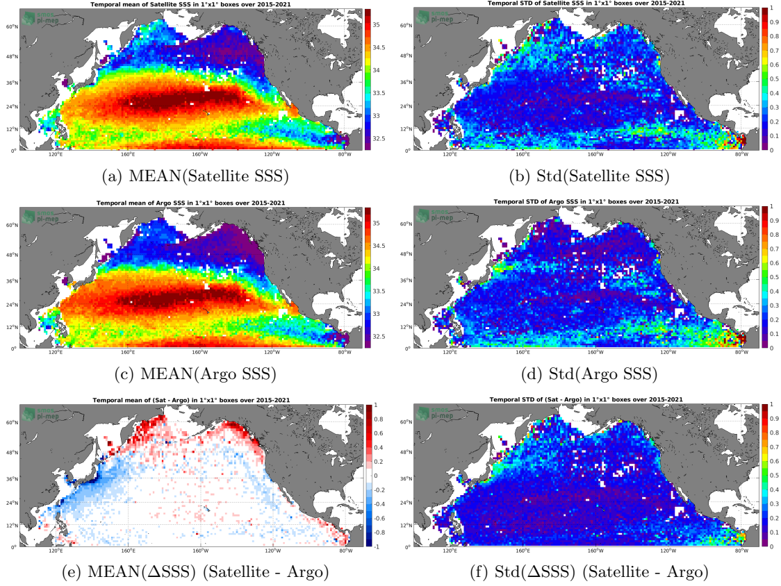
Figure 6: Temporal mean (left) and Std (right) of SSS from SMAP SSS L3 v4 - Monthly (RSS) (top), Argo (middle), and of \Delta SSS (Satellite - Argo). Only match-up pairs are used to generate these maps.
