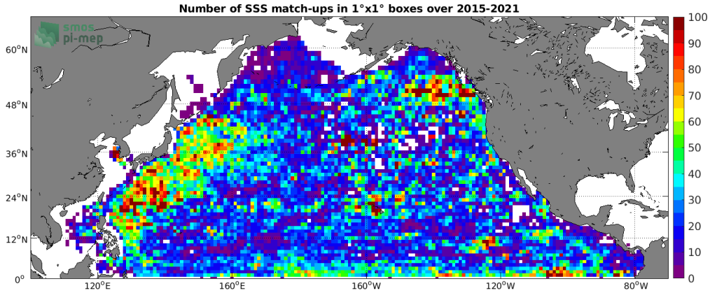
Figure 4: Number of SSS match-ups between Argo SSS and the SMAP SSS L3 v4 - Monthly (RSS) SSS product for the North Pacific Ocean Pi-MEP region over 1^\circ \times 1^\circ boxes and for the full satellite product period.
