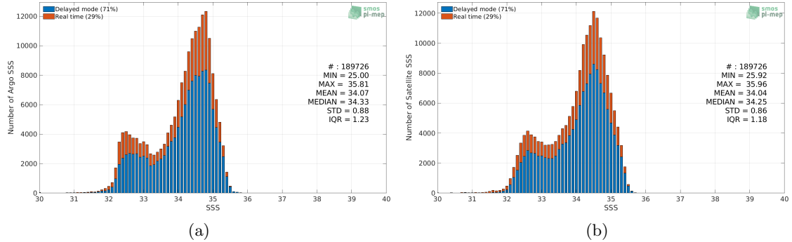
Figure 2: Histograms of SSS from Argo (a) and SMAP SSS L3 v4 - Monthly (RSS) (b) considering all match-up pairs per bins of 0.1 over the North Pacific Ocean Pi-MEP region and for the full satellite product period.
