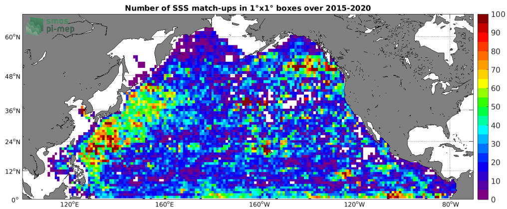
Figure 4: Number of SSS match-ups between Argo SSS and the SMAP SSS L3 v4 - Monthly (RSS) SSS product for the North Pacific Ocean Pi-MEP region over 1°x1° boxes and for the full satellite product period.
