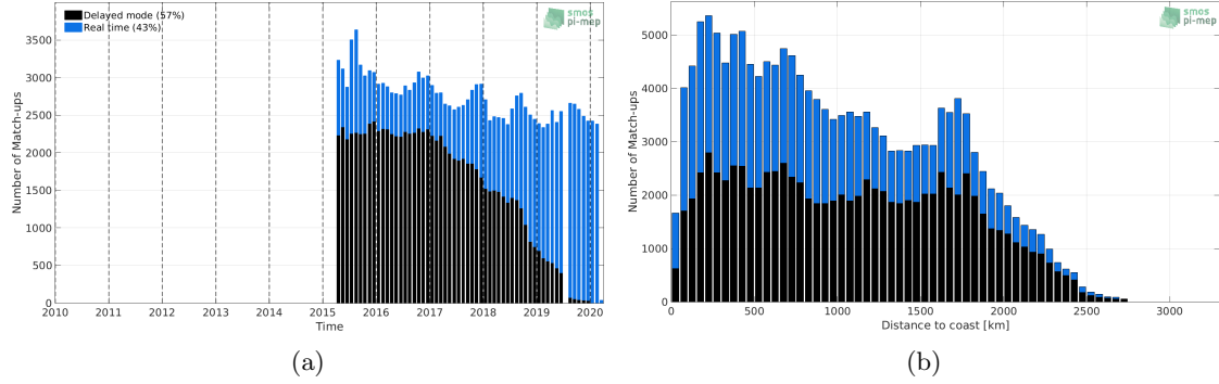
Figure 1: Number of match-ups between Argo and SMAP-L3-RSS-V4-MONTHLY SSS as a function of time (a) and as function of the distance to coast (b) over the North Pacific Ocean Pi-MEP region and for the full satellite product period.
