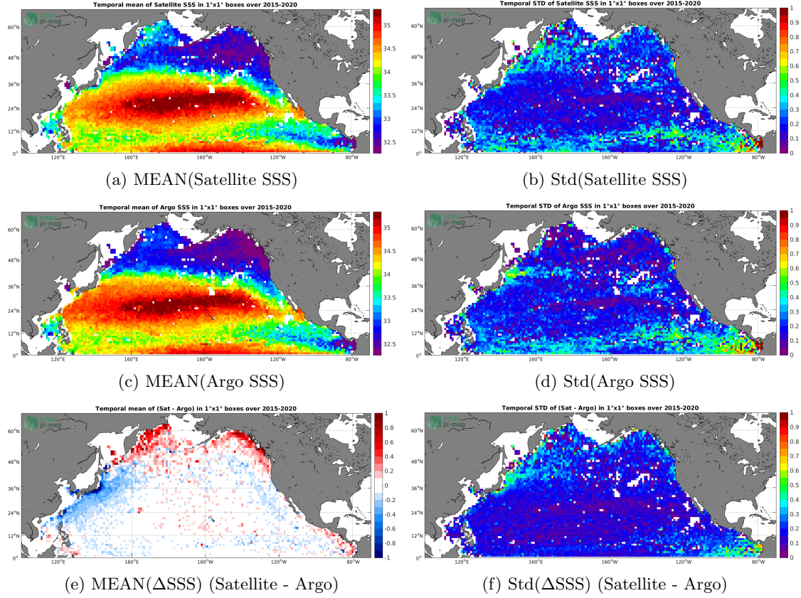
Figure 6: Temporal mean (left) and Std (right) of SSS from SMAP-L3-RSS-V4-MONTHLY (top), Argo (middle), and of \Delta SSS (Satellite - Argo). Only match-up pairs are used to generate these maps.
