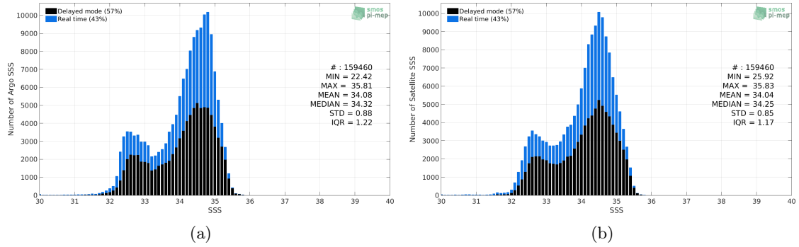
Figure 2: Histograms of SSS from Argo (a) and SMAP-L3-RSS-V4-MONTHLY (b) considering all match-up pairs per bins of 0.1 over the North Pacific Ocean Pi-MEP region and for the full satellite product period.
