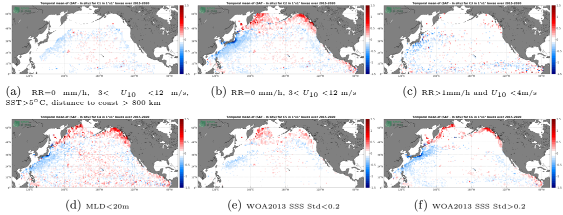
Figure 12: Temporal mean gridded over spatial boxes of size 1^\circ \times 1^\circ of \Delta SSS (SMAP-L3-RSS-V4-MONTHLY - Argo) for 6 different subdatasets corresponding to: RR=0 mm/h, 3 < U_{10} < 12 m/s, SST > 5^\circ C , distance to coast > 800 km (a), RR=0 mm/h, 3 < U_{10} < 12 m/s (b), RR > 1 mm/h and U_{10} < 4 m/s (c), MLD < 20 m (d), WOA2013 SSS Std < 0.2 (e), WOA2013 SSS Std > 0.2 (f).
