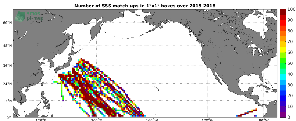
Figure 4: Number of SSS match-ups between TSG-LEGOS-DM SSS and the SMAP-L3-RSS-V3-8DAY-RUNNING-70KM SSS product for the North Pacific Ocean Pi-MEP region over 1^\circ \times 1^\circ boxes and for the full satellite product period.
