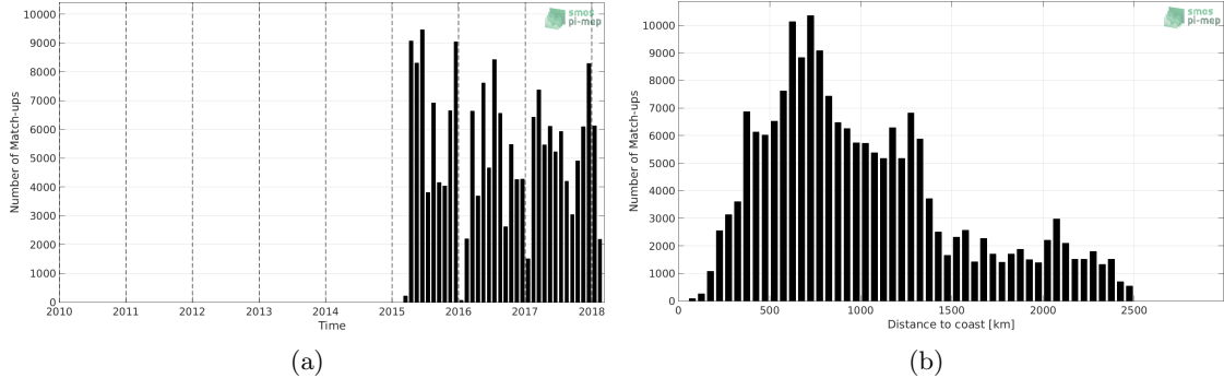
Figure 1: Number of match-ups between TSG-LEGOS-DM and SMAP-L3-RSS-V3-8DAY-RUNNING-70KM SSS as a function of time (a) and as function of the distance to coast (b) over the North Pacific Ocean Pi-MEP region and for the full satellite product period.
