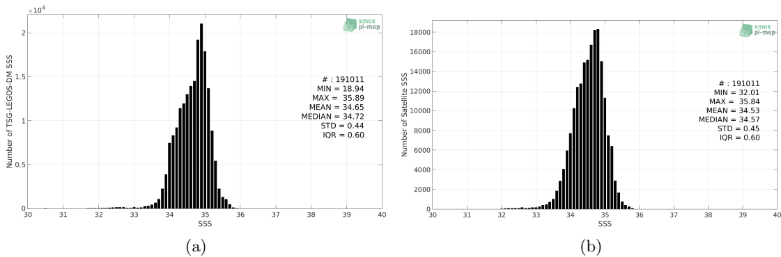
Figure 2: Histograms of SSS from TSG-LEGOS-DM (a) and SMAP-L3-RSS-V3-8DAY-RUNNING-70KM (b) considering all match-up pairs per bins of 0.1 over the North Pacific Ocean Pi-MEP region and for the full satellite product period.
