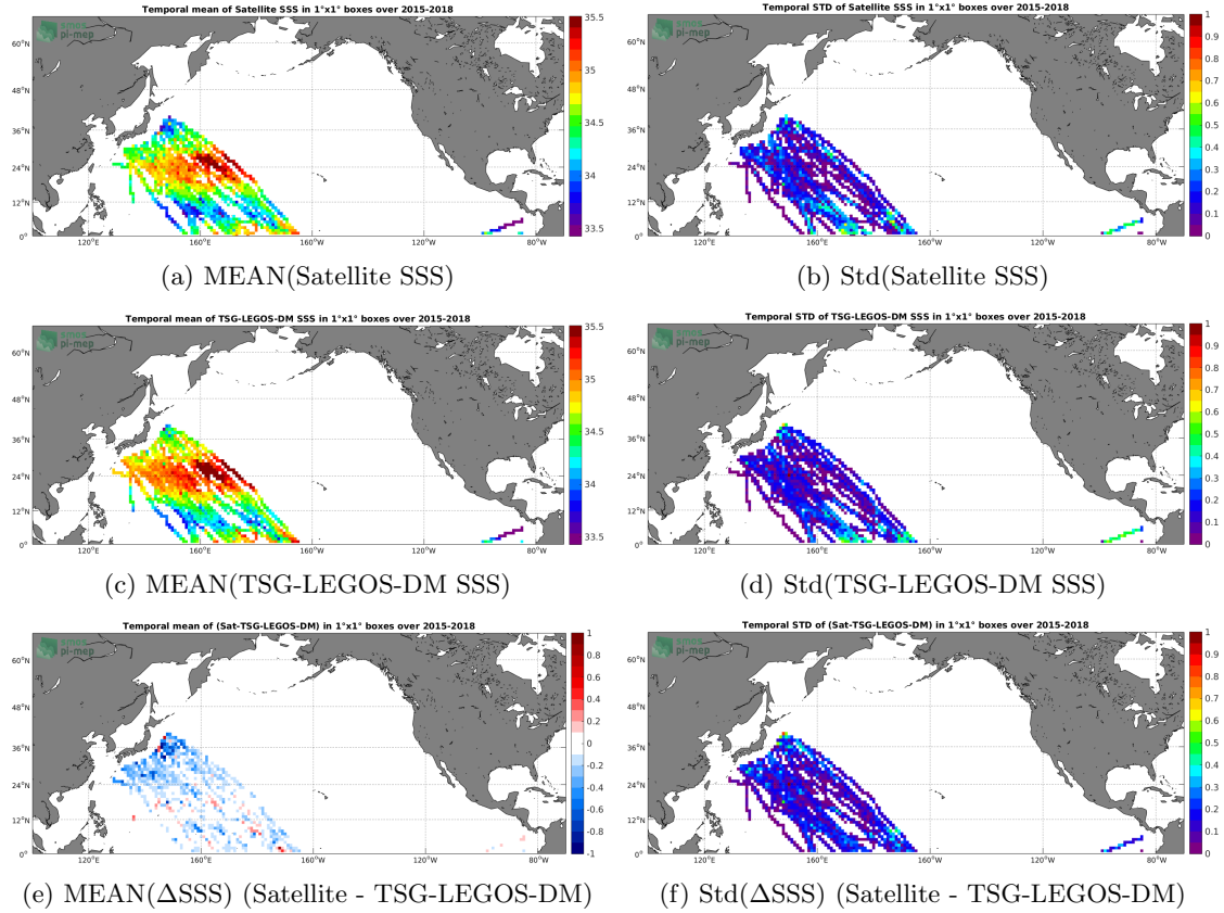
Figure 6: Temporal mean (left) and Std (right) of SSS from SMAP-L3-RSS-V3-8DAY-RUNNING-70KM (top), TSG-LEGOS-DM (middle), and of \Delta SSS (Satellite - TSG-LEGOS-DM). Only match-up pairs are used to generate these maps.
