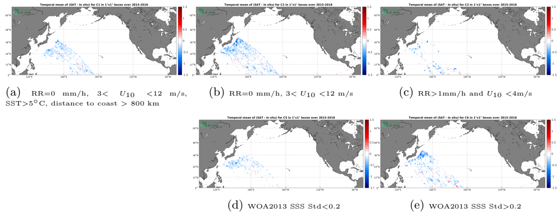
Figure 12: Temporal mean gridded over spatial boxes of size 1^\circ \times 1^\circ of \Delta SSS (SMAP-L3-RSS-V3-8DAY-RUNNING-70KM - TSG-LEGOS-DM) for 5 different subdatasets corresponding to:RR=0 mm/h, 3 < U_{10} < 12 m/s, SST > 5^\circ C , distance to coast > 800 km (a), RR=0 mm/h, 3 < U_{10} < 12 m/s (b), RR >1 mm/h and U_{10} < 4 m/s (c), WOA2013 SSS Std <0.2 (d), WOA2013 SSS Std >0.2 (e).
