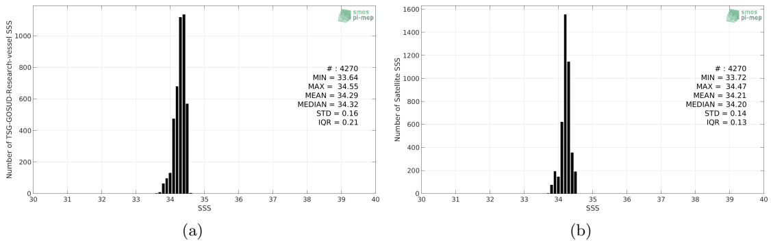
Figure 2: Histograms of SSS from TSG-GOSUD-Research-vessel (a) and SMAP-L3-RSS-V3-8DAY-RUNNING-70KM (b) considering all match-up pairs per bins of 0.1 over the North Pacific Ocean Pi-MEP region and for the full satellite product period.
