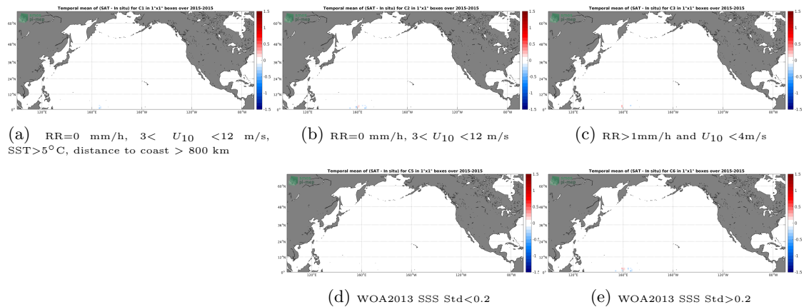
Figure 12: Temporal mean gridded over spatial boxes of size 1^\circ \times 1^\circ of \Delta SSS (SMAP-L3-RSS-V3-8DAY-RUNNING-70KM - TSG-GOSUD-Research-vessel) for 5 different subdatasets corresponding to:RR=0 mm/h, 3 < U_{10} < 12 m/s, SST >5^\circ C, distance to coast > 800 km (a), RR=0 mm/h, 3 < U_{10} < 12 m/s (b), RR >1 mm/h and U_{10} < 4 m/s (c), WOA2013 SSS Std <0.2 (d), WOA2013 SSS Std >0.2 (e).
