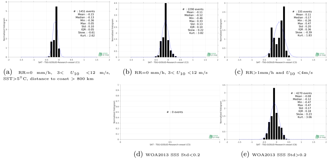
Figure 13: Normalized histogram of \Delta\text{SSS} (SMAP-L3-RSS-V3-8DAY-RUNNING-70KM - TSG-GOSUD-Research-vessel) for 5 different subdatasets corresponding to: RR=0 mm/h, 3 < U_{10} < 12 m/s, SST > 5^\circ\text{C} , distance to coast > 800 km (a), RR=0 mm/h, 3 < U_{10} < 12 m/s (b), RR > 1\text{mm/h} and U_{10} < 4\text{m/s} (c), WOA2013 SSS Std < 0.2 (d), WOA2013 SSS Std > 0.2 (e).
