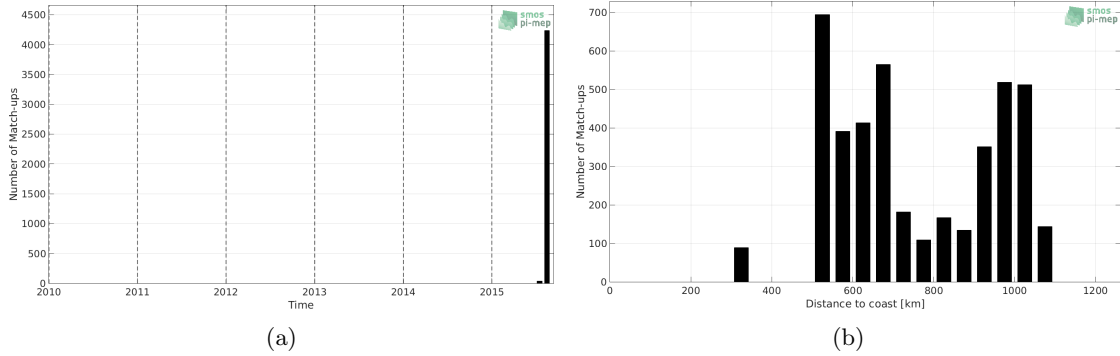
Figure 1: Number of match-ups between TSG-GOSUD-Research-vessel and SMAP-L3-RSS-V3-8DAY-RUNNING-70KM SSS as a function of time (a) and as function of the distance to coast (b) over the North Pacific Ocean Pi-MEP region and for the full satellite product period.
