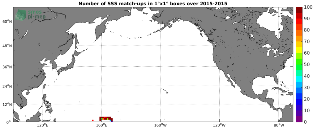
Figure 4: Number of SSS match-ups between TSG-GOSUD-Research-vessel SSS and the SMAP-L3-RSS-V3-8DAY-RUNNING-70KM SSS product for the North Pacific Ocean Pi-MEP region over 1^\circ \times 1^\circ boxes and for the full satellite product period.
