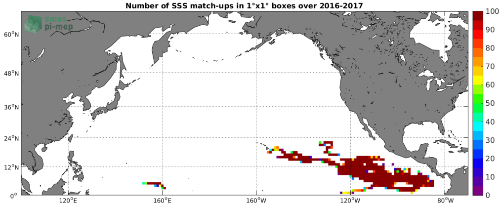
Figure 3: Number of SSS match-ups between Surface drifters SSS and the SMAP-L3-RSS-V3-8DAY-RUNNING-70KM SSS product for the North Pacific Ocean Pi-MEP region over 1^\circ \times 1^\circ boxes and for the full satellite product period.
