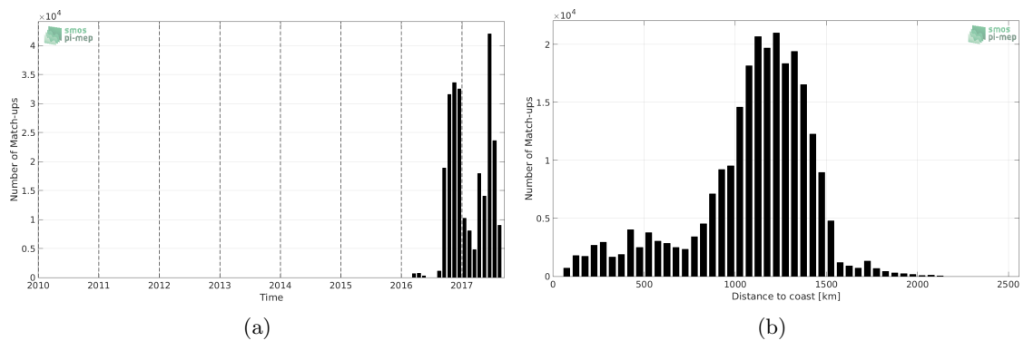
Figure 1: Number of match-ups between Surface drifters and SMAP-L3-RSS-V3-8DAY-RUNNING-70KM SSS as a function of time (a) and as function of the distance to coast (b) over the North Pacific Ocean Pi-MEP region and for the full satellite product period.
