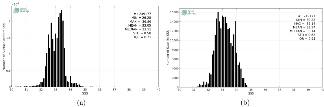
Figure 2: Histograms of SSS from Surface drifters (a) and SMAP-L3-RSS-V3-8DAY-RUNNING-70KM (b) considering all match-up pairs per bins of 0.1 over the North Pacific Ocean Pi-MEP region and for the full satellite product period.
