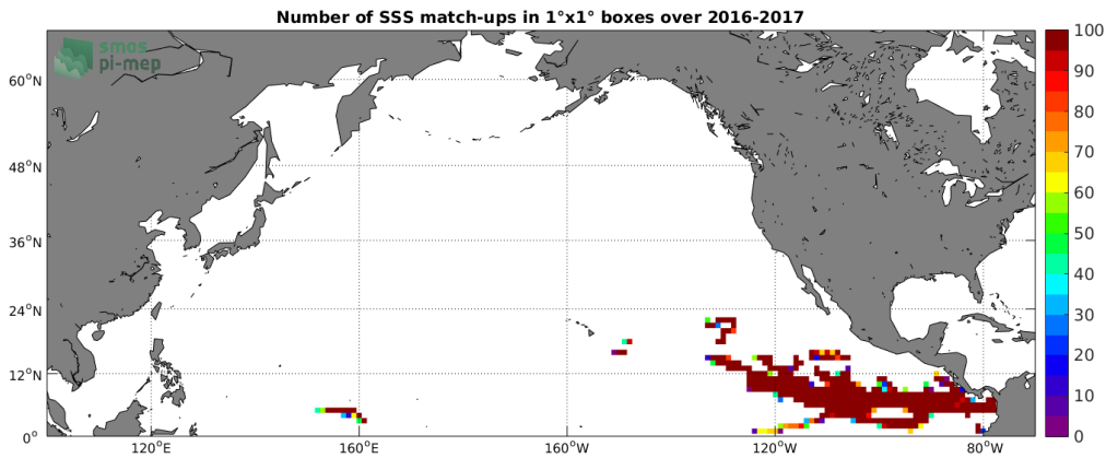
Figure 3: Number of SSS match-ups between Surface drifters SSS and the SMAP-L3-RSS-V3-8DAY-RUNNING-70KM SSS product for the North Pacific Ocean Pi-MEP region over 1°x1° boxes and for the full satellite product period.
