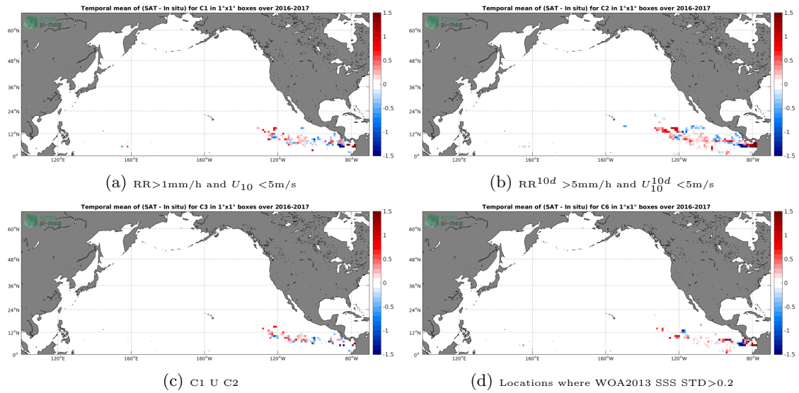
Figure 11: Temporal mean gridded over spatial boxes of size 1^\circ \times 1^\circ of \Delta SSS (SMAP-L3-RSS-V3-8DAY-RUNNING-70KM - Surface drifters) for 4 different subdatasets corresponding to: RR > 1\text{mm/h} and U_{10} < 5\text{m/s} (a), RR^{10d} > 5\text{mm/h} and U_{10}^{10d} < 5\text{m/s} (b), C1 U C2 (c), Locations where WOA2013 SSS STD > 0.2 (d).
