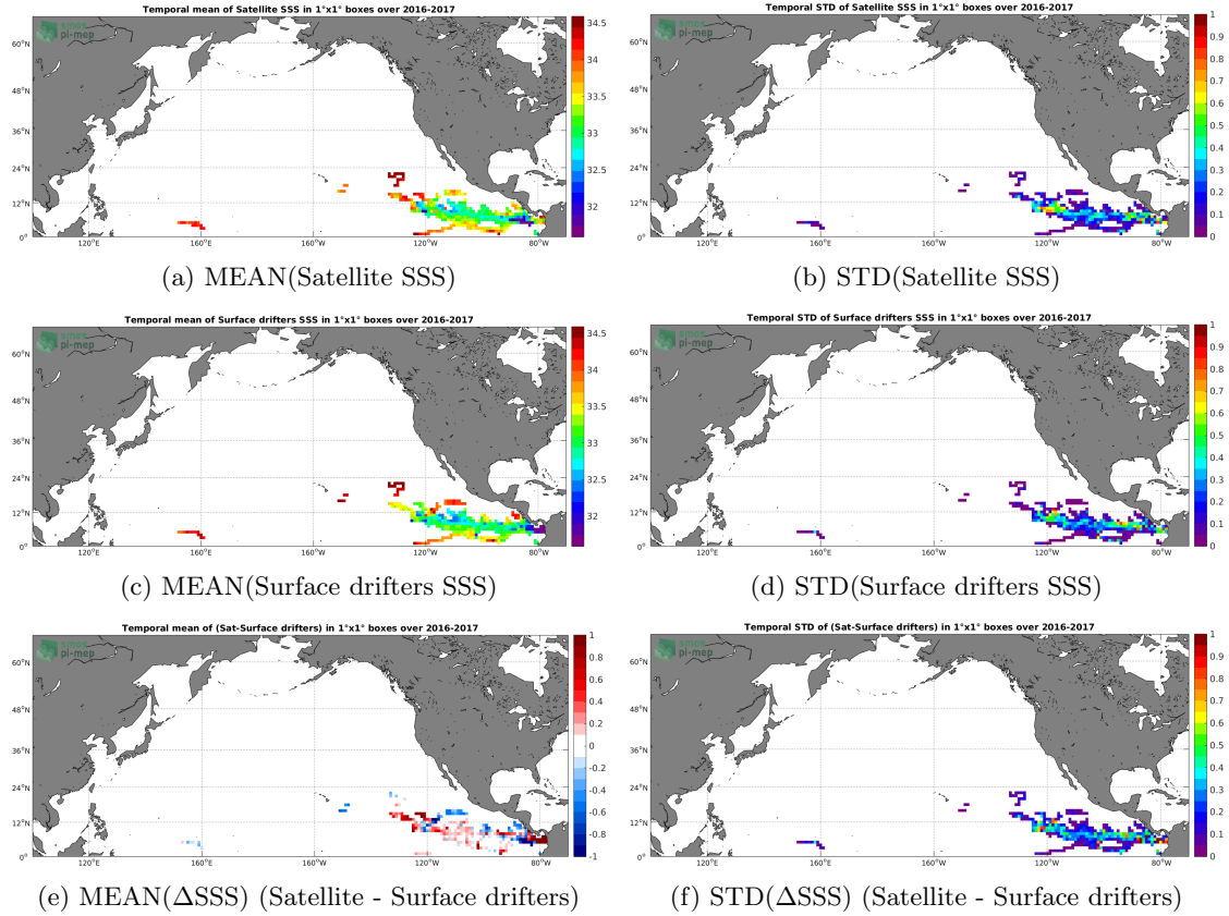
Figure 5: Temporal mean (left) and STD (right) of SSS from SMAP-L3-RSS-V3-8DAY-RUNNING-70KM (top), Surface drifters (middle), and of \Delta SSS (Satellite - Surface drifters). Only match-up pairs are used to generate these maps.
