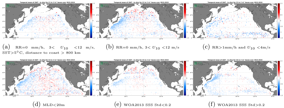
Figure 12: Temporal mean gridded over spatial boxes of size 1^\circ \times 1^\circ of \Delta SSS (SMAP-L3-RSS-V3-8DAY-RUNNING-70KM - Argo) for 6 different subdatasets corresponding to:RR=0 mm/h, 3 < U_{10} < 12 m/s, SST >5^\circ C, distance to coast > 800 km (a), RR=0 mm/h, 3 < U_{10} < 12 m/s (b), RR >1 mm/h and U_{10} < 4 m/s (c),MLD <20 m (d),WOA2013 SSS Std <0.2 (e),WOA2013 SSS Std >0.2 (f).
