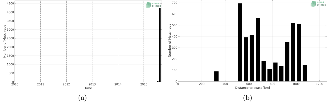
Figure 1: Number of match-ups between TSG-GOSUD-Research-vessel and SMAP-L3-RSS-V3-8DAY-RUNNING-40KM SSS as a function of time (a) and as function of the distance to coast (b) over the North Pacific Ocean Pi-MEP region and for the full satellite product period.
