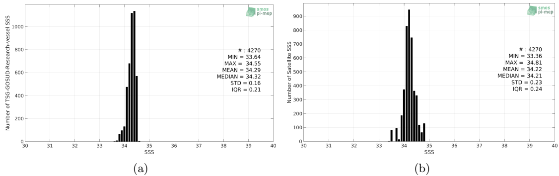
Figure 2: Histograms of SSS from TSG-GOSUD-Research-vessel (a) and SMAP-L3-RSS-V3-8DAY-RUNNING-40KM (b) considering all match-up pairs per bins of 0.1 over the North Pacific Ocean Pi-MEP region and for the full satellite product period.
