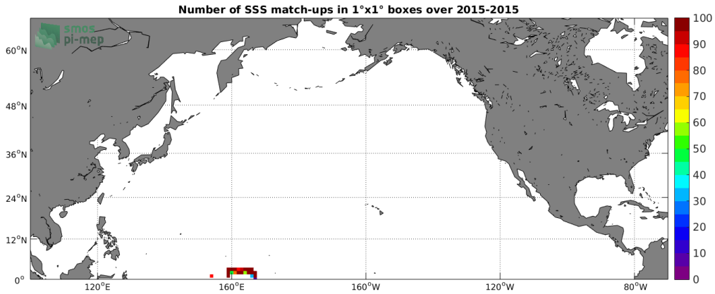
Figure 4: Number of SSS match-ups between TSG-GOSUD-Research-vessel SSS and the SMAP-L3-RSS-V3-8DAY-RUNNING-40KM SSS product for the North Pacific Ocean Pi-MEP region over 1^\circ \times 1^\circ boxes and for the full satellite product period.
