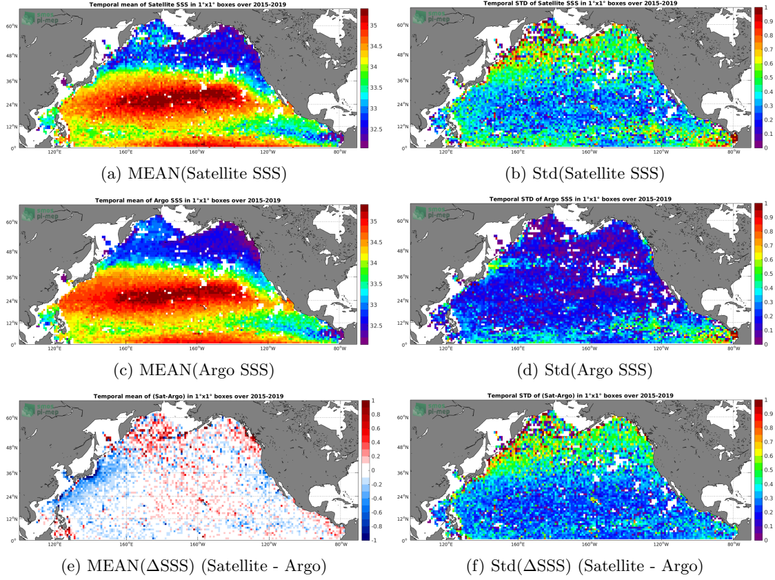
Figure 6: Temporal mean (left) and Std (right) of SSS from SMAP-L3-RSS-V3-8DAY-RUNNING-40KM (top), Argo (middle), and of \Delta SSS (Satellite - Argo). Only match-up pairs are used to generate these maps.
