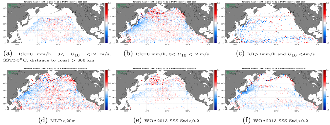
Figure 12: Temporal mean gridded over spatial boxes of size 1^\circ \times 1^\circ of \Delta SSS (SMAP-L3-RSS-V3-8DAY-RUNNING-40KM - Argo) for 6 different subdatasets corresponding to: RR=0 mm/h, 3 < U_{10} < 12 m/s, SST > 5^\circ C , distance to coast > 800 km (a), RR=0 mm/h, 3 < U_{10} < 12 m/s (b), RR > 1 mm/h and U_{10} < 4 m/s (c), MLD < 20 m (d), WOA2013 SSS Std < 0.2 (e), WOA2013 SSS Std > 0.2 (f).
