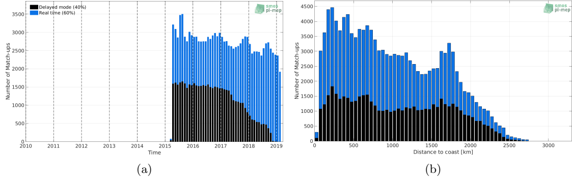
Figure 1: Number of match-ups between Argo and SMAP-L3-RSS-V3-8DAY-RUNNING-40KM SSS as a function of time (a) and as function of the distance to coast (b) over the North Pacific Ocean Pi-MEP region and for the full satellite product period.
