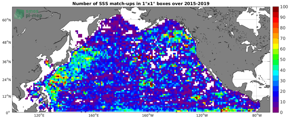
Figure 4: Number of SSS match-ups between Argo SSS and the SMAP-L3-RSS-V3-8DAY-RUNNING-40KM SSS product for the North Pacific Ocean Pi-MEP region over 1°x1° boxes and for the full satellite product period.
