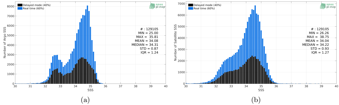
Figure 2: Histograms of SSS from Argo (a) and SMAP-L3-RSS-V3-8DAY-RUNNING-40KM (b) considering all match-up pairs per bins of 0.1 over the North Pacific Ocean Pi-MEP region and for the full satellite product period.
