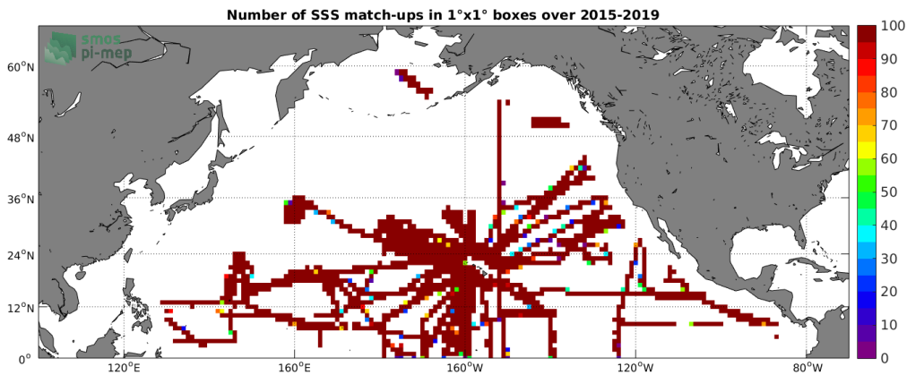
Figure 4: Number of SSS match-ups between TSG-SAMOS SSS and the SMAP-L3-RSS-V3-MONTHLY-70KM SSS product for the North Pacific Ocean Pi-MEP region over 1^\circ \times 1^\circ boxes and for the full satellite product period.
