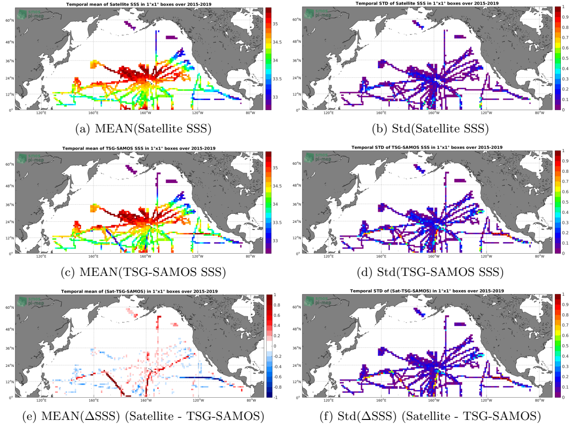
Figure 6: Temporal mean (left) and Std (right) of SSS from SMAP-L3-RSS-V3-MONTHLY-70KM (top), TSG-SAMOS (middle), and of \Delta SSS (Satellite - TSG-SAMOS). Only match-up pairs are used to generate these maps.
