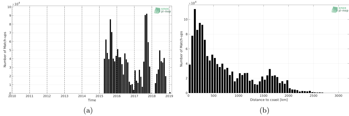
Figure 1: Number of match-ups between TSG-SAMOS and SMAP-L3-RSS-V3-MONTHLY-70KM SSS as a function of time (a) and as function of the distance to coast (b) over the North Pacific Ocean Pi-MEP region and for the full satellite product period.
