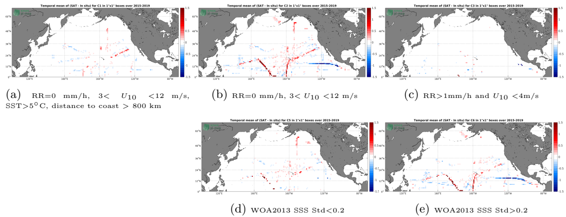
Figure 12: Temporal mean gridded over spatial boxes of size 1^\circ \times 1^\circ of \Delta SSS (SMAP-L3-RSS-V3-MONTHLY-70KM - TSG-SAMOS) for 5 different subdatasets corresponding to:RR=0 mm/h, 3 < U_{10} < 12 m/s, SST >5^\circ\text{C} , distance to coast > 800 km (a), RR=0 mm/h, 3 < U_{10} < 12 m/s (b), RR >1 mm/h and U_{10} < 4 m/s (c), WOA2013 SSS Std <0.2 (d), WOA2013 SSS Std >0.2 (e).
