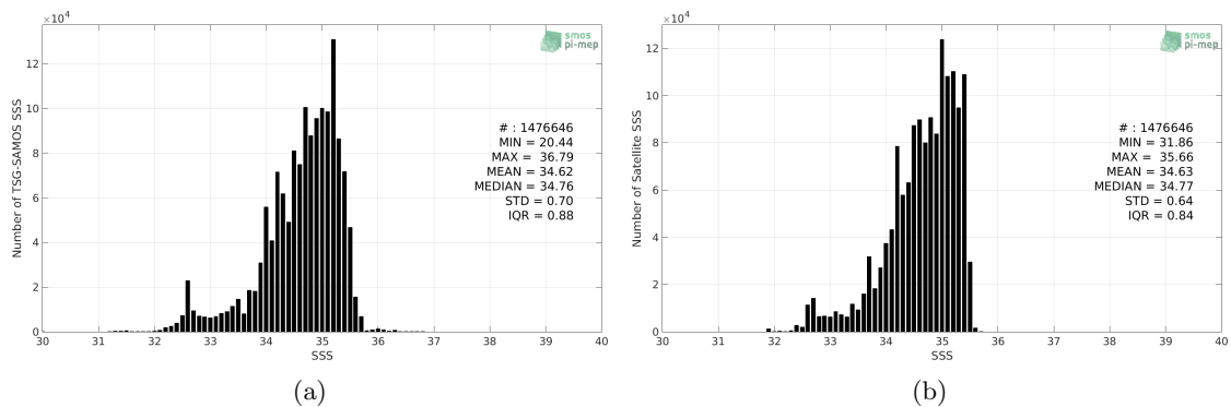
Figure 2: Histograms of SSS from TSG-SAMOS (a) and SMAP-L3-RSS-V3-MONTHLY-70KM (b) considering all match-up pairs per bins of 0.1 over the North Pacific Ocean Pi-MEP region and for the full satellite product period.
