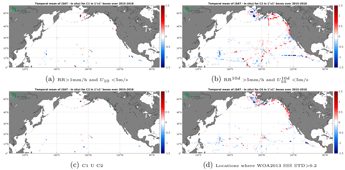
Figure 12: Temporal mean gridded over spatial boxes of size 1^\circ \times 1^\circ of \Delta SSS (SMAP-L3-RSS-V3-MONTHLY-70KM - TSG-SAMOS) for 4 different subdatasets corresponding to: RR > 1\text{mm/h} and U_{10} < 5\text{m/s} (a), RR^{10d} > 5\text{mm/h} and U_{10}^{10d} < 5\text{m/s} (b), C1 U C2 (c), Locations where WOA2013 SSS STD > 0.2 (d).
