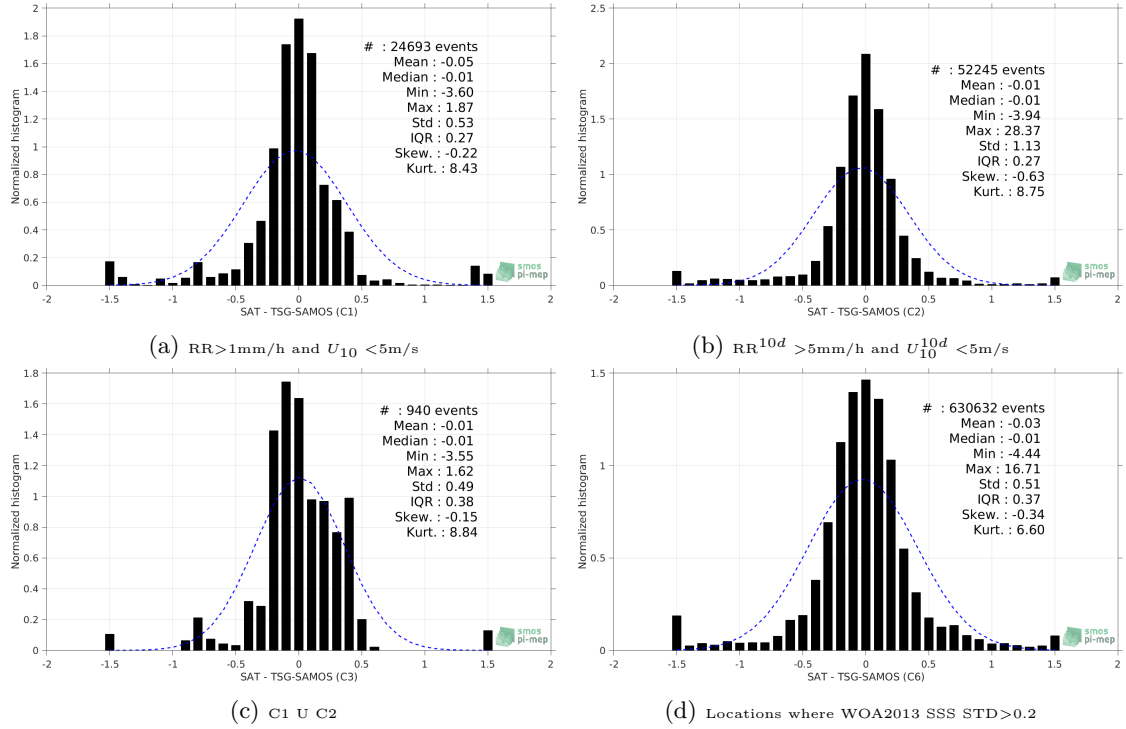
Figure 13: Normalized histogram of \Delta SSS (SMAP-L3-RSS-V3-MONTHLY-70KM - TSG-SAMOS) for 6 different subdatasets corresponding to: RR > 1\text{mm/h} and U_{10} < 5\text{m/s} (a), RR^{10d} > 5\text{mm/h} and U_{10}^{10d} < 5\text{m/s} (b), C1 U C2 (c), Locations where WOA2013 SSS STD > 0.2 (d).
