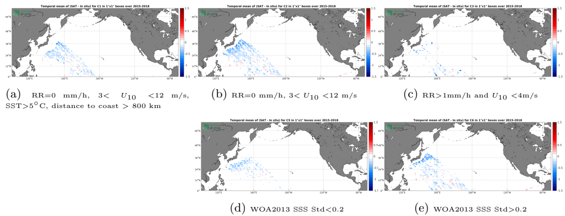
Figure 12: Temporal mean gridded over spatial boxes of size 1^\circ \times 1^\circ of \Delta SSS (SMAP-L3-RSS-V3-MONTHLY-70KM - TSG-LEGOS-DM) for 5 different subdatasets corresponding to:RR=0 mm/h, 3 < U_{10} < 12 m/s, SST > 5^\circ\text{C} , distance to coast > 800 km (a), RR=0 mm/h, 3 < U_{10} < 12 m/s (b), RR > 1 mm/h and U_{10} < 4 m/s (c), WOA2013 SSS Std < 0.2 (d), WOA2013 SSS Std > 0.2 (e).
