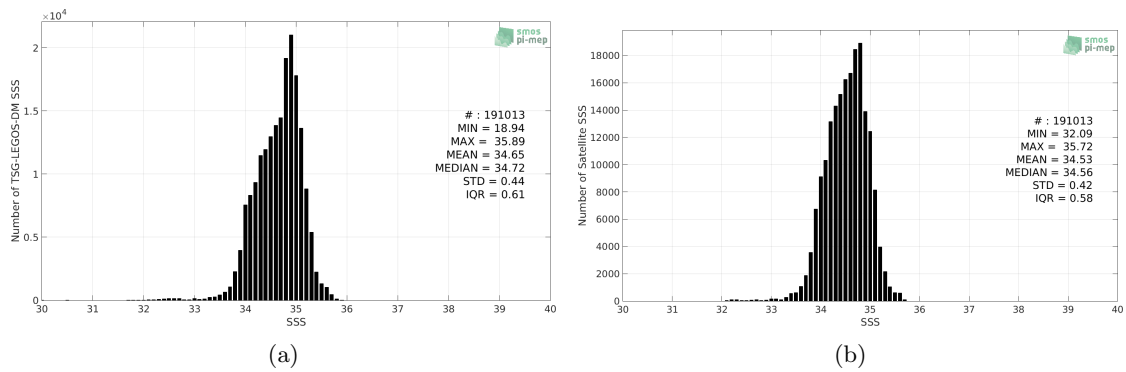
Figure 2: Histograms of SSS from TSG-LEGOS-DM (a) and SMAP-L3-RSS-V3-MONTHLY-70KM (b) considering all match-up pairs per bins of 0.1 over the North Pacific Ocean Pi-MEP region and for the full satellite product period.
