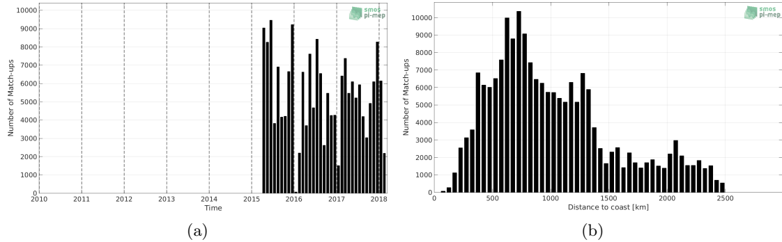
Figure 1: Number of match-ups between TSG-LEGOS-DM and SMAP-L3-RSS-V3-MONTHLY-70KM SSS as a function of time (a) and as function of the distance to coast (b) over the North Pacific Ocean Pi-MEP region and for the full satellite product period.
