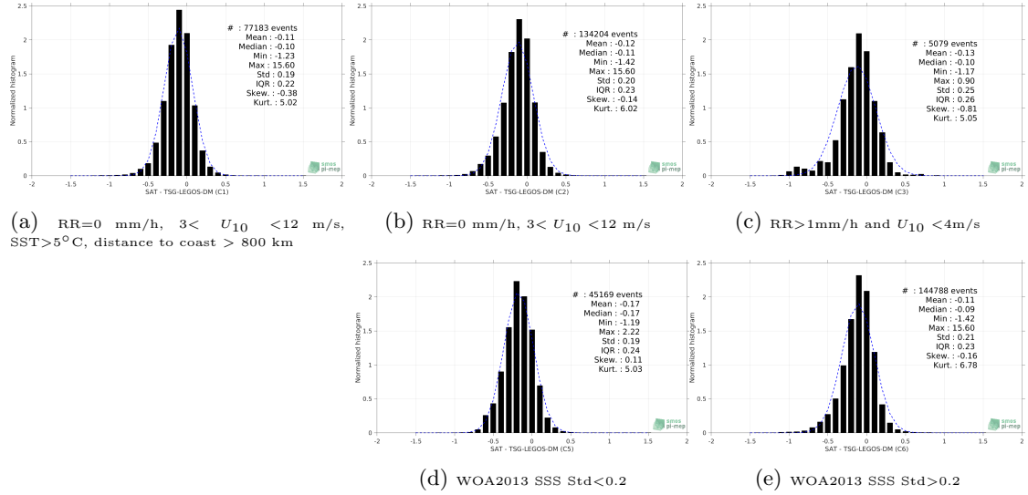
Figure 13: Normalized histogram of \Delta\text{SSS} (SMAP-L3-RSS-V3-MONTHLY-70KM - TSG-LEGOS-DM) for 5 different subdatasets corresponding to: RR=0 mm/h, 3 < U_{10} < 12 m/s, SST>5°C, distance to coast > 800 km (a), RR=0 mm/h, 3 < U_{10} < 12 m/s (b), RR>1mm/h and U_{10} < 4 m/s (c), WOA2013 SSS Std<0.2 (d), WOA2013 SSS Std>0.2 (e).
