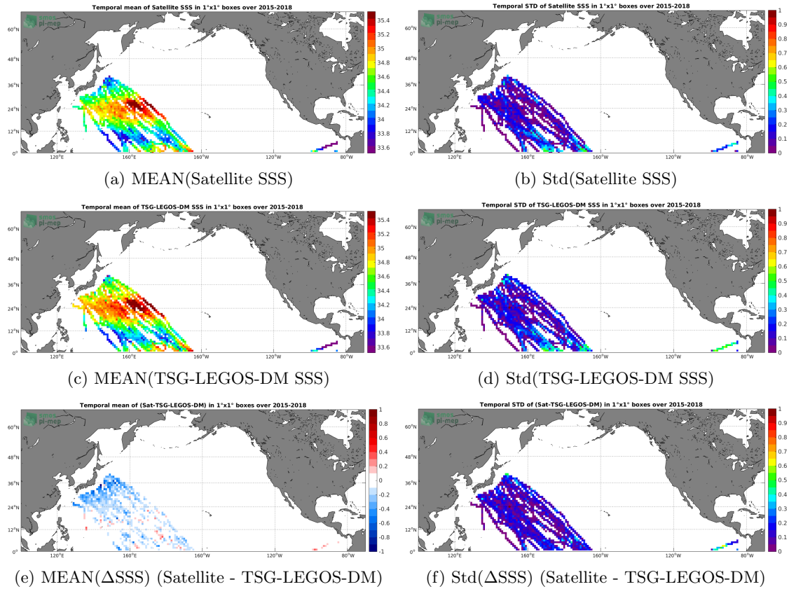
Figure 6: Temporal mean (left) and Std (right) of SSS from SMAP-L3-RSS-V3-MONTHLY-70KM (top), TSG-LEGOS-DM (middle), and of \Delta SSS (Satellite - TSG-LEGOS-DM). Only match-up pairs are used to generate these maps.
