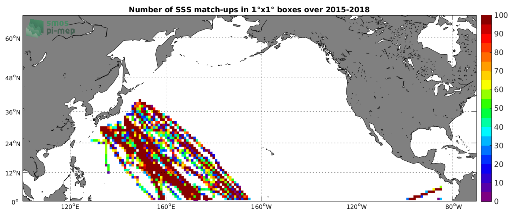
Figure 4: Number of SSS match-ups between TSG-LEGOS-DM SSS and the SMAP-L3-RSS-V3-MONTHLY-70KM SSS product for the North Pacific Ocean Pi-MEP region over 1^\circ \times 1^\circ boxes and for the full satellite product period.
