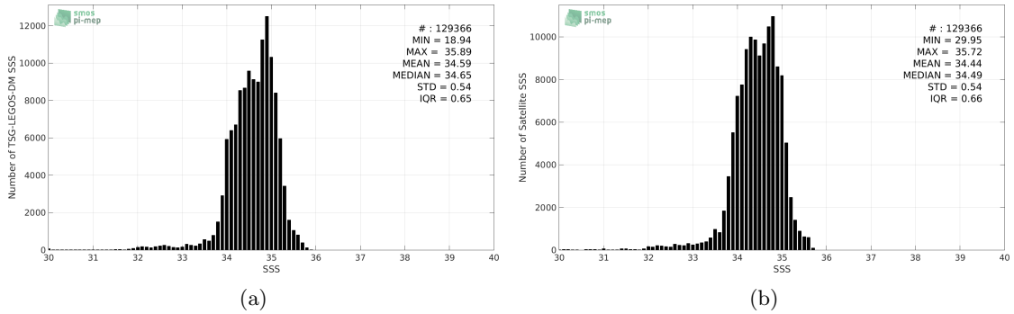
Figure 2: Histograms of SSS from TSG-LEGOS-DM (a) and SMAP-L3-RSS-V3-MONTHLY-70KM (b) considering all match-up pairs per bins of 0.1 over the North Pacific Ocean Pi-MEP region and for the full satellite product period.
