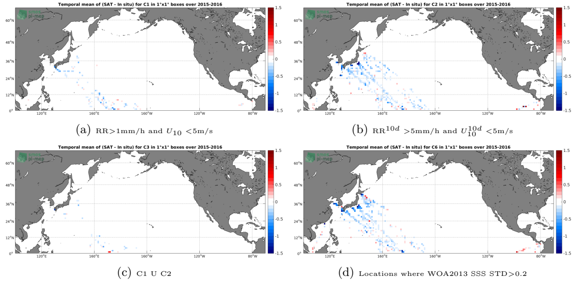
Figure 12: Temporal mean gridded over spatial boxes of size 1^\circ \times 1^\circ of \Delta SSS (SMAP-L3-RSS-V3-MONTHLY-70KM - TSG-LEGOS-DM) for 4 different subdatasets corresponding to: RR > 1\text{mm/h} and U_{10} < 5\text{m/s} (a), RR^{10d} > 5\text{mm/h} and U_{10}^{10d} < 5\text{m/s} (b), C1 U C2 (c), Locations where WOA2013 SSS STD > 0.2 (d).
