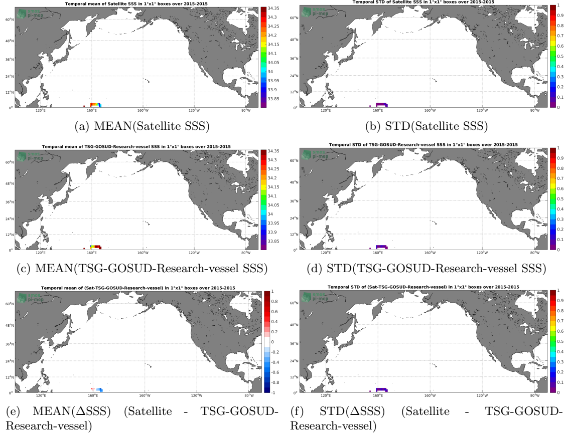
Figure 6: Temporal mean (left) and STD (right) of SSS from SMAP-L3-RSS-V3-MONTHLY-70KM (top), TSG-GOSUD-Research-vessel (middle), and of \Delta SSS (Satellite - TSG-GOSUD-Research-vessel). Only match-up pairs are used to generate these maps.
