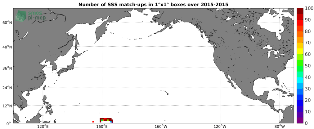
Figure 4: Number of SSS match-ups between TSG-GOSUD-Research-vessel SSS and the SMAP-L3-RSS-V3-MONTHLY-70KM SSS product for the North Pacific Ocean Pi-MEP region over 1^\circ \times 1^\circ boxes and for the full satellite product period.
