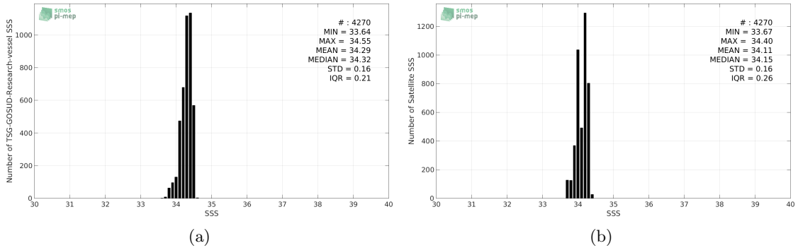
Figure 2: Histograms of SSS from TSG-GOSUD-Research-vessel (a) and SMAP-L3-RSS-V3-MONTHLY-70KM (b) considering all match-up pairs per bins of 0.1 over the North Pacific Ocean Pi-MEP region and for the full satellite product period.
