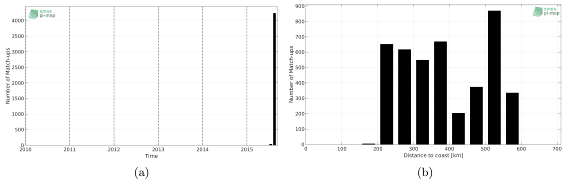
Figure 1: Number of match-ups between TSG-GOSUD-Research-vessel and SMAP-L3-RSS-V3-MONTHLY-70KM SSS as a function of time (a) and as function of the distance to coast (b) over the North Pacific Ocean Pi-MEP region and for the full satellite product period.
