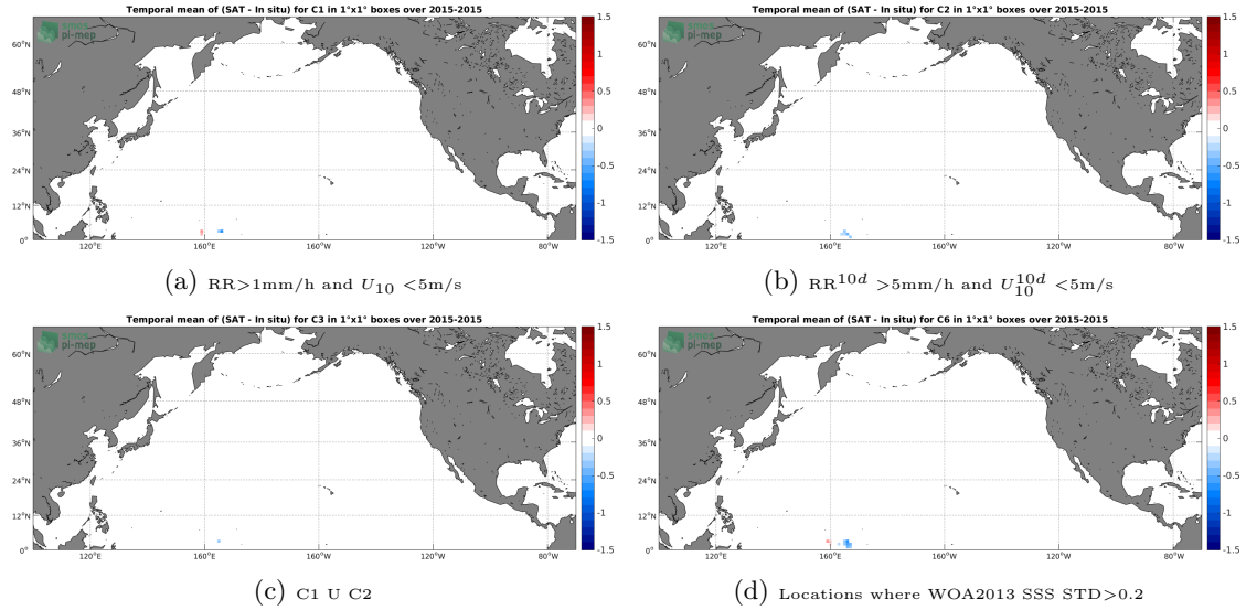
Figure 12: Temporal mean gridded over spatial boxes of size 1^\circ \times 1^\circ of \Delta SSS (SMAP-L3-RSS-V3-MONTHLY-70KM - TSG-GOSUD-Research-vessel) for 4 different subdatasets corresponding to: RR > 1\text{mm/h} and U_{10} < 5\text{m/s} (a), RR^{10d} > 5\text{mm/h} and U_{10}^{10d} < 5\text{m/s} (b), C1 U C2 (c), Locations where WOA2013 SSS STD > 0.2 (d).
