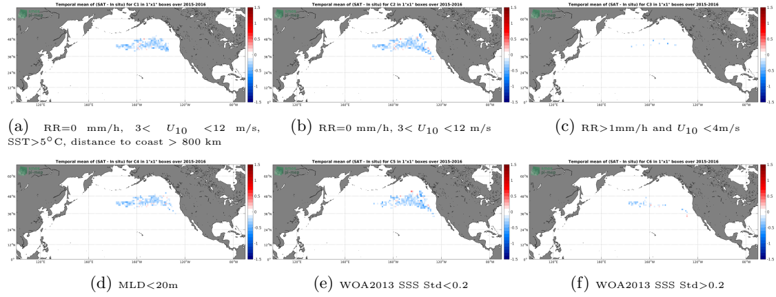
Figure 12: Temporal mean gridded over spatial boxes of size 1^\circ \times 1^\circ of \Delta SSS (SMAP-L3-RSS-V3-MONTHLY-70KM - Sea mammals) for 6 different subdatasets corresponding to: RR=0 mm/h, 3 < U_{10} < 12 m/s, SST >5^\circ\text{C} , distance to coast > 800 km (a), RR=0 mm/h, 3 < U_{10} < 12 m/s (b), RR>1\text{mm/h} and U_{10} < 4\text{m/s} (c), MLD<20\text{m} (d), WOA2013 SSS Std <0.2 (e), WOA2013 SSS Std >0.2 (f).
