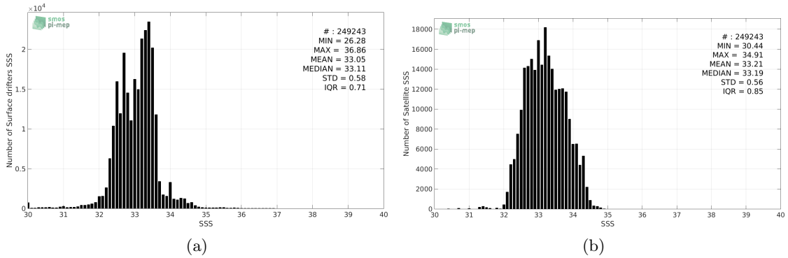
Figure 2: Histograms of SSS from Surface drifters (a) and SMAP-L3-RSS-V3-MONTHLY-70KM (b) considering all match-up pairs per bins of 0.1 over the North Pacific Ocean Pi-MEP region and for the full satellite product period.
