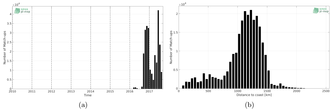
Figure 1: Number of match-ups between Surface drifters and SMAP-L3-RSS-V3-MONTHLY-70KM SSS as a function of time (a) and as function of the distance to coast (b) over the North Pacific Ocean Pi-MEP region and for the full satellite product period.
