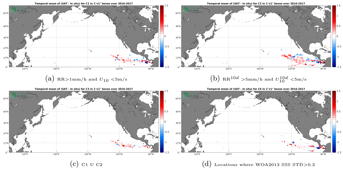
Figure 11: Temporal mean gridded over spatial boxes of size 1^\circ \times 1^\circ of \Delta SSS (SMAP-L3-RSS-V3-MONTHLY-70KM - Surface drifters) for 4 different subdatasets corresponding to: RR > 1\text{mm/h} and U_{10} < 5\text{m/s} (a), RR^{10d} > 5\text{mm/h} and U_{10}^{10d} < 5\text{m/s} (b), C1 U C2 (c), Locations where WOA2013 SSS STD > 0.2 (d).
