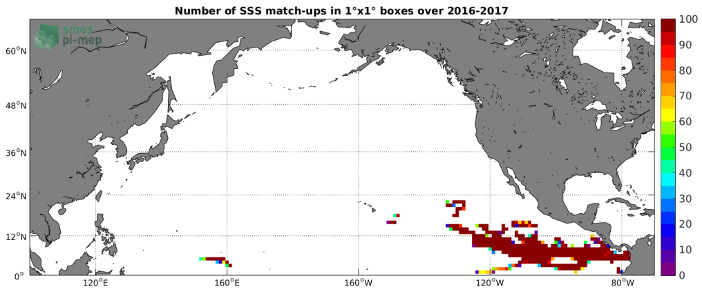
Figure 3: Number of SSS match-ups between Surface drifters SSS and the SMAP-L3-RSS-V3-MONTHLY-70KM SSS product for the North Pacific Ocean Pi-MEP region over 1°x1° boxes and for the full satellite product period.
