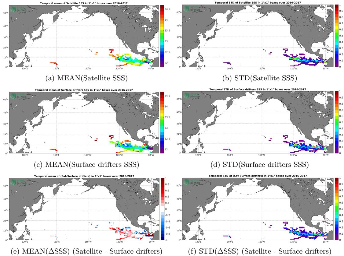
Figure 5: Temporal mean (left) and STD (right) of SSS from SMAP-L3-RSS-V3-MONTHLY-70KM (top), Surface drifters (middle), and of \Delta SSS (Satellite - Surface drifters). Only match-up pairs are used to generate these maps.
