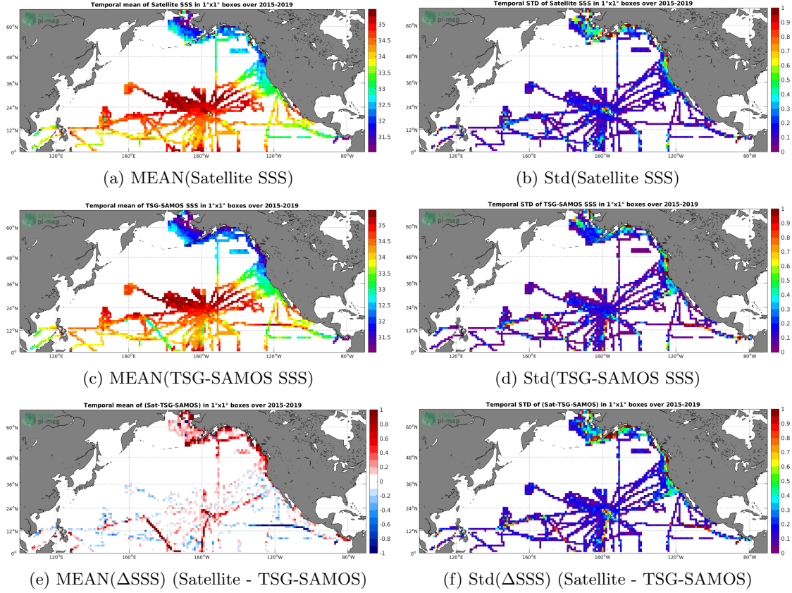
Figure 6: Temporal mean (left) and Std (right) of SSS from SMAP-L3-RSS-V3-MONTHLY-0.25DEG-40KM (top), TSG-SAMOS (middle), and of \Delta SSS (Satellite - TSG-SAMOS). Only match-up pairs are used to generate these maps.
