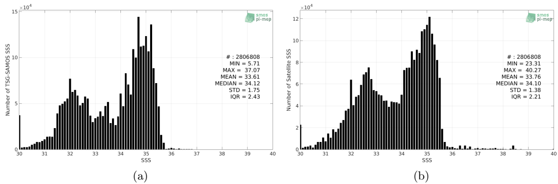
Figure 2: Histograms of SSS from TSG-SAMOS (a) and SMAP-L3-RSS-V3-MONTHLY-0.25DEG-40KM (b) considering all match-up pairs per bins of 0.1 over the North Pacific Ocean Pi-MEP region and for the full satellite product period.
