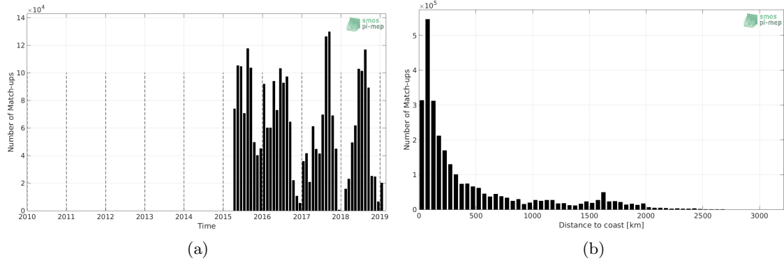
Figure 1: Number of match-ups between TSG-SAMOS and SMAP-L3-RSS-V3-MONTHLY-0.25DEG-40KM SSS as a function of time (a) and as function of the distance to coast (b) over the North Pacific Ocean Pi-MEP region and for the full satellite product period.
