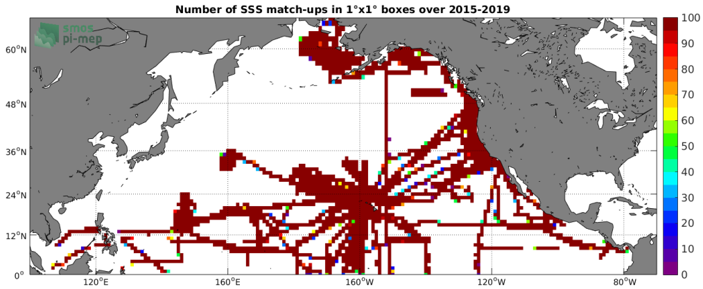
Figure 4: Number of SSS match-ups between TSG-SAMOS SSS and the SMAP-L3-RSS-V3-MONTHLY-0.25DEG-40KM SSS product for the North Pacific Ocean Pi-MEP region over 1^\circ \times 1^\circ boxes and for the full satellite product period.
