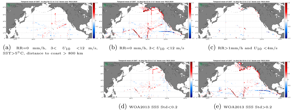
Figure 12: Temporal mean gridded over spatial boxes of size 1^\circ \times 1^\circ of \Delta SSS (SMAP-L3-RSS-V3-MONTHLY-0.25DEG-40KM - TSG-SAMOS) for 5 different subdatasets corresponding to: RR=0 mm/h, 3 < U_{10} < 12 m/s, SST > 5^\circ\text{C} , distance to coast > 800 km (a), RR=0 mm/h, 3 < U_{10} < 12 m/s (b), RR > 1\text{mm/h} and U_{10} < 4\text{m/s} (c), WOA2013 SSS Std < 0.2 (d), WOA2013 SSS Std > 0.2 (e).
