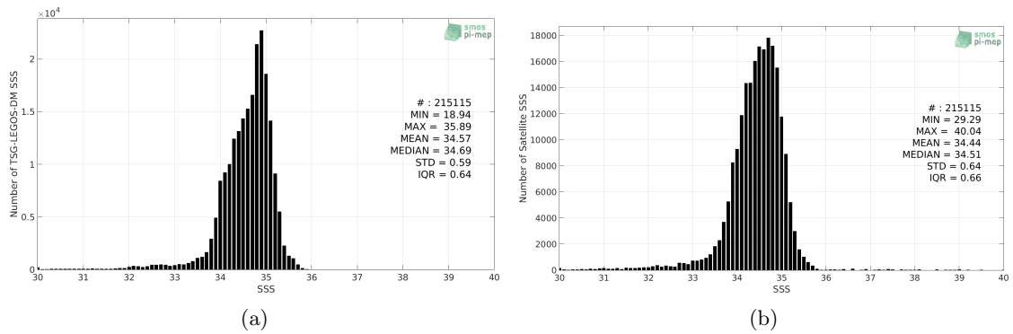
Figure 2: Histograms of SSS from TSG-LEGOS-DM (a) and SMAP-L3-RSS-V3-MONTHLY-0.25DEG-40KM (b) considering all match-up pairs per bins of 0.1 over the North Pacific Ocean Pi-MEP region and for the full satellite product period.
