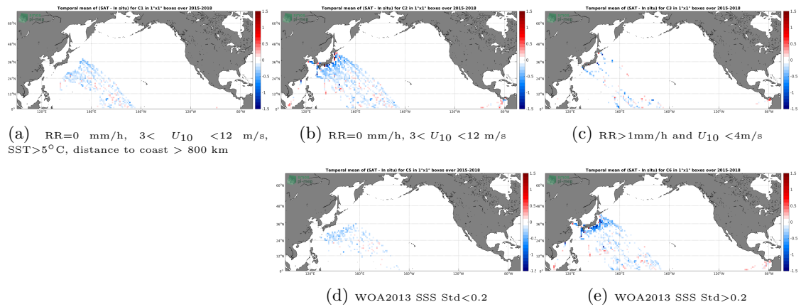
Figure 12: Temporal mean gridded over spatial boxes of size 1^\circ \times 1^\circ of \Delta SSS (SMAP-L3-RSS-V3-MONTHLY-0.25DEG-40KM - TSG-LEGOS-DM) for 5 different subdatasets corresponding to:RR=0 mm/h, 3 < U_{10} < 12 m/s, SST >5^\circ C, distance to coast > 800 km (a), RR=0 mm/h, 3 < U_{10} < 12 m/s (b), RR >1 mm/h and U_{10} < 4 m/s (c), WOA2013 SSS Std <0.2 (d), WOA2013 SSS Std >0.2 (e).
