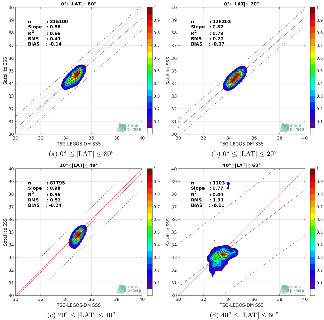
Figure 9: Contour maps of the concentration of SMAP-L3-RSS-V3-MONTHLY-0.25DEG-40KM SSS (y-axis) versus TSG-LEGOS-DM SSS (x-axis) at match-up pairs for different latitude bands. For each plot, the red line shows x=y . The black thin and dashed lines indicate a linear fit through the data cloud and the \pm 95\% confidence levels, respectively. The number match-up pairs n , the slope and R^2 coefficient of the linear fit, the root mean square (RMS) and the mean bias between satellite and in situ data are indicated for each latitude band in each plots.
