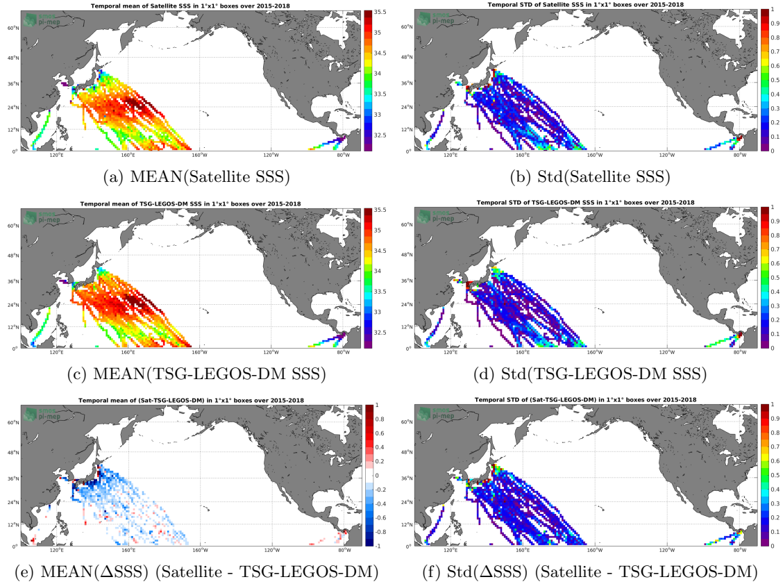
Figure 6: Temporal mean (left) and Std (right) of SSS from SMAP-L3-RSS-V3-MONTHLY-0.25DEG-40KM (top), TSG-LEGOS-DM (middle), and of \Delta SSS (Satellite - TSG-LEGOS-DM). Only match-up pairs are used to generate these maps.
