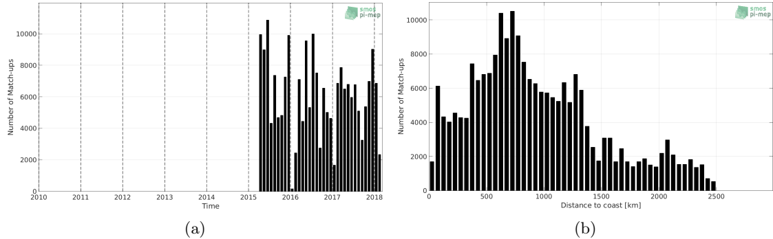
Figure 1: Number of match-ups between TSG-LEGOS-DM and SMAP-L3-RSS-V3-MONTHLY-0.25DEG-40KM SSS as a function of time (a) and as function of the distance to coast (b) over the North Pacific Ocean Pi-MEP region and for the full satellite product period.
