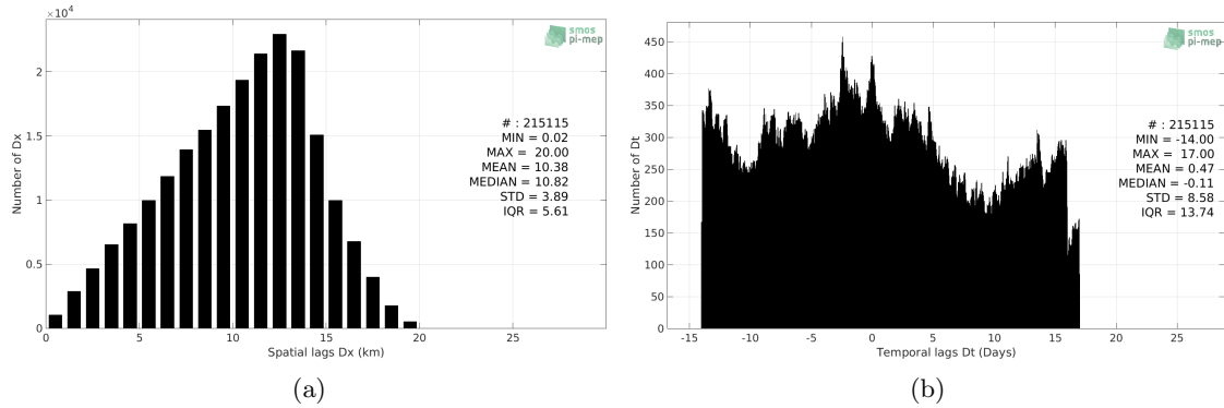
Figure 5: Histograms of the spatial (a) and temporal (b) lags between the time of the TSG-LEGOS-DM measurements and the date of the corresponding SMAP-L3-RSS-V3-MONTHLY-0.25DEG-40KM SSS product.
