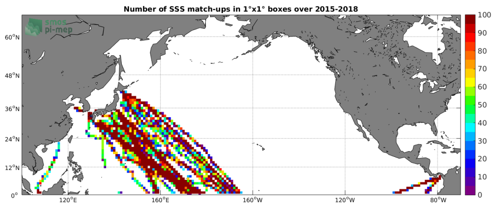
Figure 4: Number of SSS match-ups between TSG-LEGOS-DM SSS and the SMAP-L3-RSS-V3-MONTHLY-0.25DEG-40KM SSS product for the North Pacific Ocean Pi-MEP region over 1^\circ \times 1^\circ boxes and for the full satellite product period.
