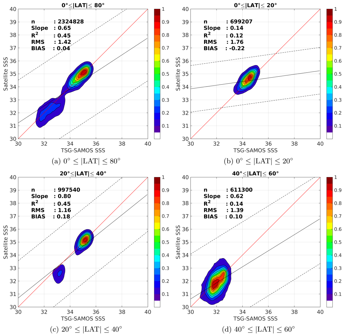
Figure 9: Contour maps of the concentration of SMAP-L3-RSS-V2-8DAY-RUNNING-40KM SSS (y-axis) versus TSG-SAMOS SSS (x-axis) at match-up pairs for different latitude bands. For each plot, the red line shows x=y . The black thin and dashed lines indicate a linear fit through the data cloud and the \pm 95\% confidence levels, respectively. The number match-up pairs n , the slope and R^2 coefficient of the linear fit, the root mean square (RMS) and the mean bias between satellite and in situ data are indicated for each latitude band in each plots.
