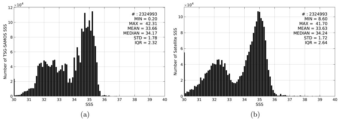
Figure 2: Histograms of SSS from TSG-SAMOS (a) and SMAP-L3-RSS-V2-8DAY-RUNNING-40KM (b) considering all match-up pairs per bins of 0.1 over the North Pacific Ocean Pi-MEP region and for the full satellite product period.
