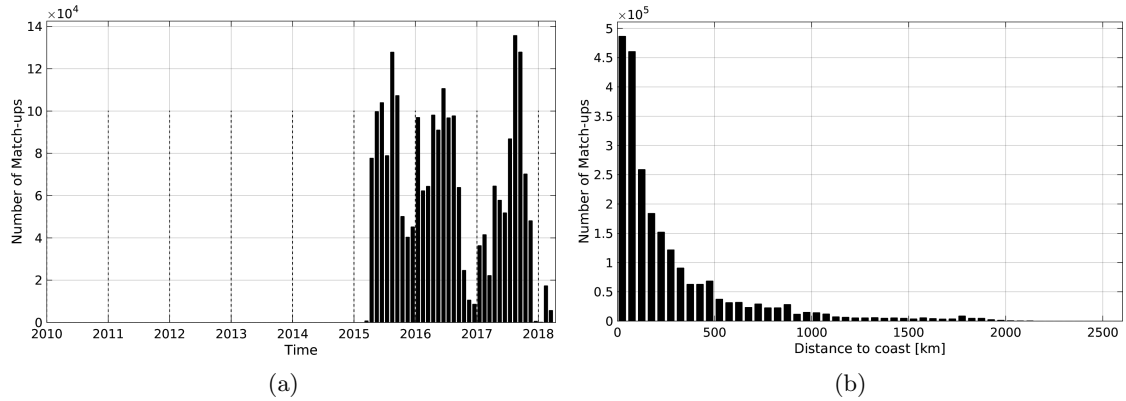
Figure 1: Number of match-ups between TSG-SAMOS and SMAP-L3-RSS-V2-8DAY-RUNNING-40KM SSS as a function of time (a) and as function of the distance to coast (b) over the North Pacific Ocean Pi-MEP region and for the full satellite product period.
