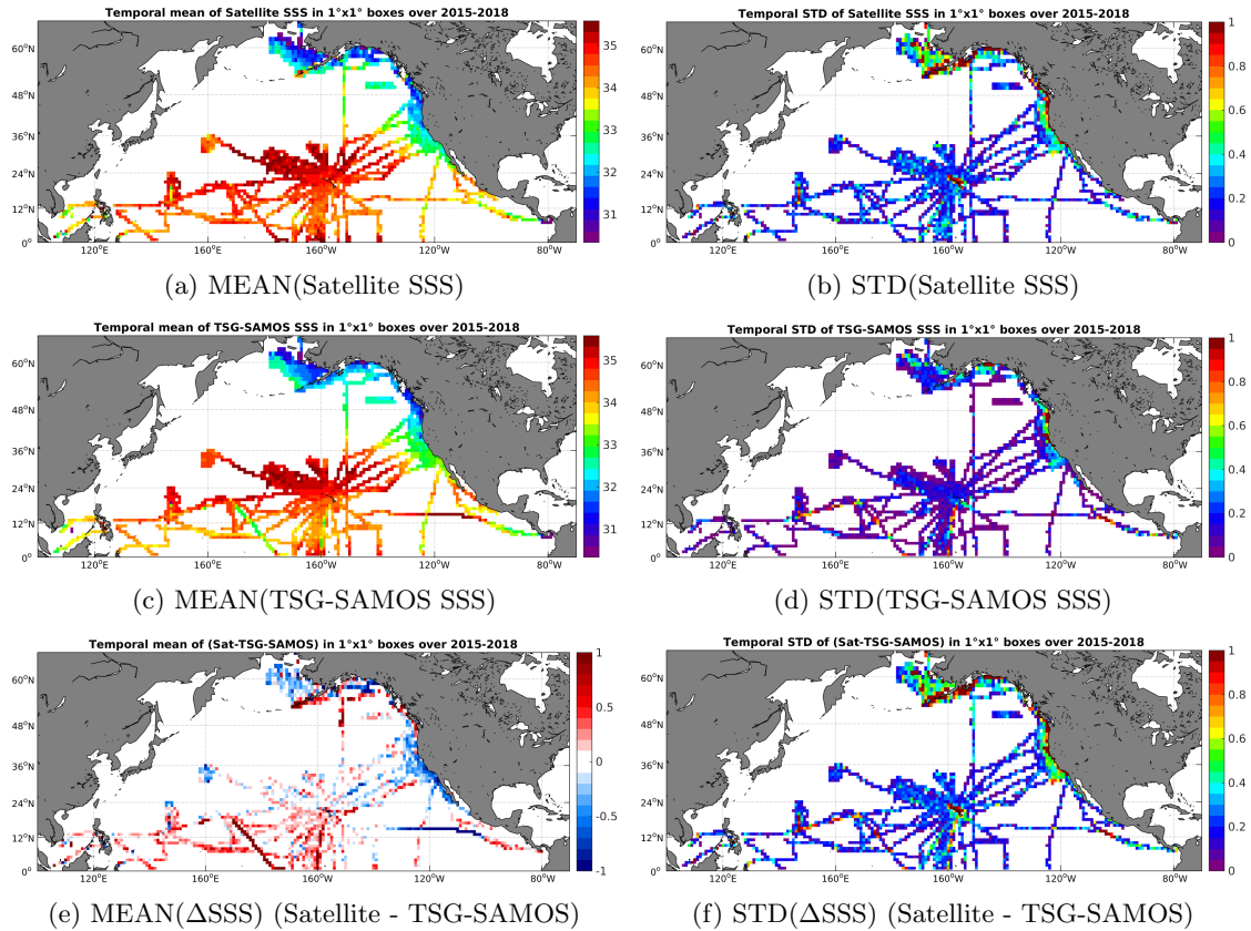
Figure 6: Temporal mean (left) and STD (right) of SSS from SMAP-L3-RSS-V2-8DAY-RUNNING-40KM (top), TSG-SAMOS (middle), and of \Delta SSS (Satellite - TSG-SAMOS). Only match-up pairs are used to generate these maps.
