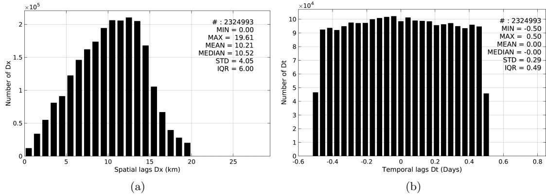
Figure 5: Histograms of the spatial (a) and temporal (b) lags between the time of the TSG-SAMOS measurements and the date of the corresponding SMAP-L3-RSS-V2-8DAY-RUNNING-40KM SSS product.
