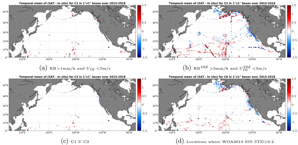
Figure 12: Temporal mean gridded over spatial boxes of size 1^\circ \times 1^\circ of \Delta SSS (SMAP-L3-RSS-V2-8DAY-RUNNING-40KM - TSG-SAMOS) for 4 different subdatasets corresponding to: RR > 1\text{mm/h} and U_{10} < 5\text{m/s} (a), RR^{10d} > 5\text{mm/h} and U_{10}^{10d} < 5\text{m/s} (b), C1 U C2 (c), Locations where WOA2013 SSS STD > 0.2 (d).
