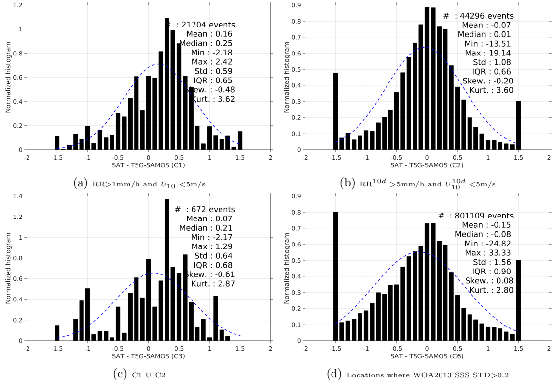
Figure 13: Normalized histogram of \Delta SSS (SMAP-L3-RSS-V2-8DAY-RUNNING-40KM - TSG-SAMOS) for 6 different subdatasets corresponding to: RR > 1\text{mm/h} and U_{10} < 5\text{m/s} (a), RR^{10d} > 5\text{mm/h} and U_{10}^{10d} < 5\text{m/s} (b), C1 U C2 (c), Locations where WOA2013 SSS STD > 0.2 (d).
