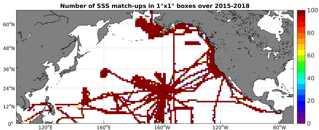
Figure 4: Number of SSS match-ups between TSG-SAMOS SSS and the SMAP-L3-RSS-V2-8DAY-RUNNING-40KM SSS product for the North Pacific Ocean Pi-MEP region over 1^\circ \times 1^\circ boxes and for the full satellite product period.
