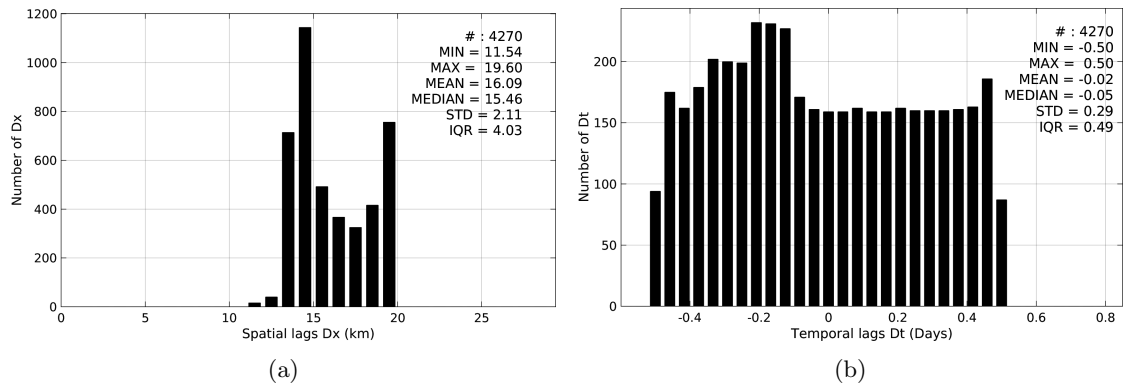
Figure 5: Histograms of the spatial (a) and temporal (b) lags between the time of the TSG-GOSUD-Research-vessel measurements and the date of the corresponding SMAP-L3-RSS-V2-8DAY-RUNNING-40KM SSS product.
