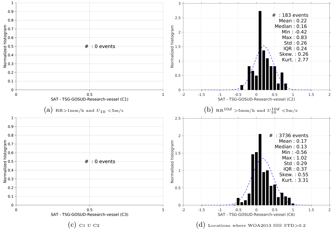
Figure 13: Normalized histogram of \Delta\text{SSS} (SMAP-L3-RSS-V2-8DAY-RUNNING-40KM - TSG-GOSUD-Research-vessel) for 6 different subdatasets corresponding to: RR > 1\text{mm/h} and U_{10} < 5\text{m/s} (a), RR^{10d} > 5\text{mm/h} and U_{10}^{10d} < 5\text{m/s} (b), C1 \cup C2 (c), Locations where WOA2013 SSS STD > 0.2 (d).
