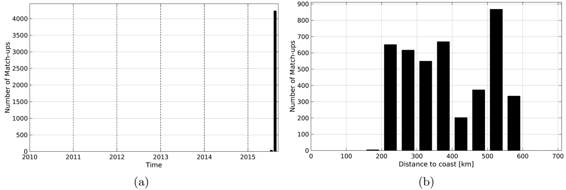
Figure 1: Number of match-ups between TSG-GOSUD-Research-vessel and SMAP-L3-RSS-V2-8DAY-RUNNING-40KM SSS as a function of time (a) and as function of the distance to coast (b) over the North Pacific Ocean Pi-MEP region and for the full satellite product period.
