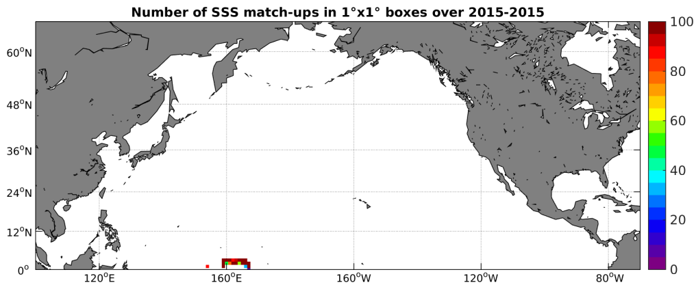
Figure 4: Number of SSS match-ups between TSG-GOSUD-Research-vessel SSS and the SMAP-L3-RSS-V2-8DAY-RUNNING-40KM SSS product for the North Pacific Ocean Pi-MEP region over 1^\circ \times 1^\circ boxes and for the full satellite product period.
