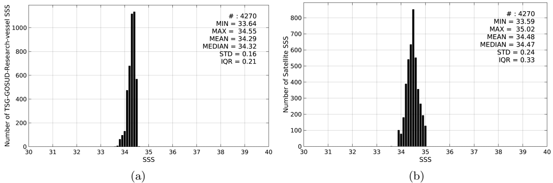
Figure 2: Histograms of SSS from TSG-GOSUD-Research-vessel (a) and SMAP-L3-RSS-V2-8DAY-RUNNING-40KM (b) considering all match-up pairs per bins of 0.1 over the North Pacific Ocean Pi-MEP region and for the full satellite product period.
