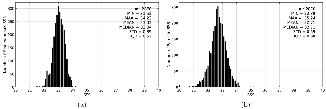
Figure 2: Histograms of SSS from Sea mammals (a) and SMAP-L3-RSS-V2-8DAY-RUNNING-40KM (b) considering all match-up pairs per bins of 0.1 over the North Pacific Ocean Pi-MEP region and for the full satellite product period.
