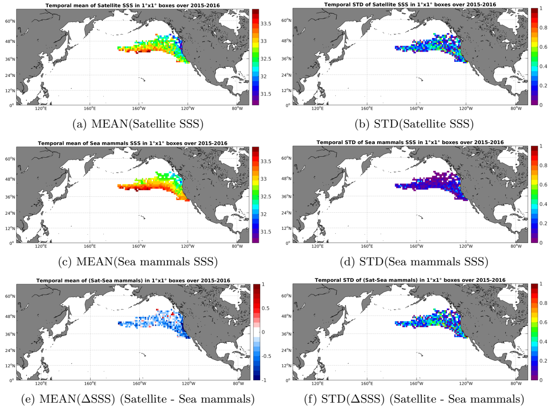
Figure 6: Temporal mean (left) and STD (right) of SSS from SMAP-L3-RSS-V2-8DAY-RUNNING-40KM (top), Sea mammals (middle), and of \Delta SSS (Satellite - Sea mammals). Only match-up pairs are used to generate these maps.
