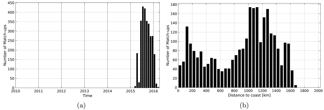
Figure 1: Number of match-ups between Sea mammals and SMAP-L3-RSS-V2-8DAY-RUNNING-40KM SSS as a function of time (a) and as function of the distance to coast (b) over the North Pacific Ocean Pi-MEP region and for the full satellite product period.
