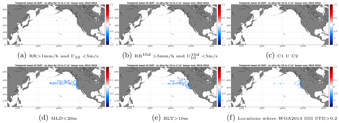
Figure 12: Temporal mean gridded over spatial boxes of size 1^\circ \times 1^\circ of \Delta SSS (SMAP-L3-RSS-V2-8DAY-RUNNING-40KM - Sea mammals) for 6 different subdatasets corresponding to:RR>1mm/h and U_{10} < 5 m/s (a), RR^{10d} > 5 mm/h and U_{10}^{10d} < 5 m/s (b), C1 U C2 (c),MLD<20m (d),BLT>10m (e),Locations where WOA2013 SSS STD>0.2 (f).
