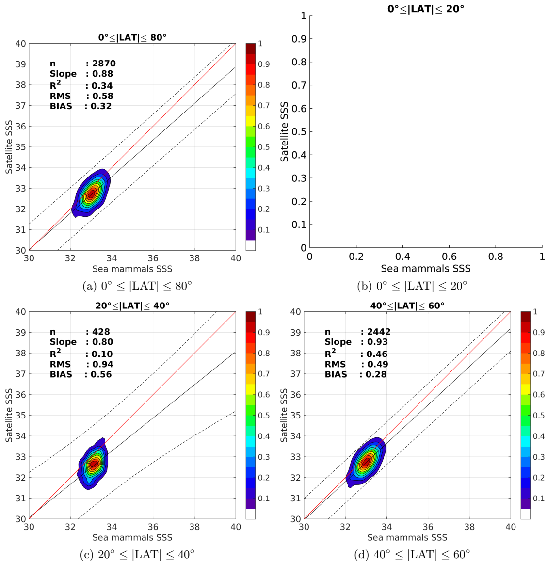
Figure 9: Contour maps of the concentration of SMAP-L3-RSS-V2-8DAY-RUNNING-40KM SSS (y-axis) versus Sea mammals SSS (x-axis) at match-up pairs for different latitude bands. For each plot, the red line shows x=y . The black thin and dashed lines indicate a linear fit through the data cloud and the \pm 95\% confidence levels, respectively. The number match-up pairs n , the slope and R^2 coefficient of the linear fit, the root mean square (RMS) and the mean bias between satellite and in situ data are indicated for each latitude band in each plots.
