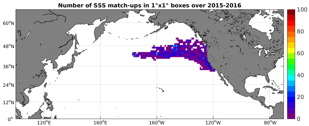
Figure 4: Number of SSS match-ups between Sea mammals SSS and the SMAP-L3-RSS-V2-8DAY-RUNNING-40KM SSS product for the North Pacific Ocean Pi-MEP region over 1^\circ \times 1^\circ boxes and for the full satellite product period.
