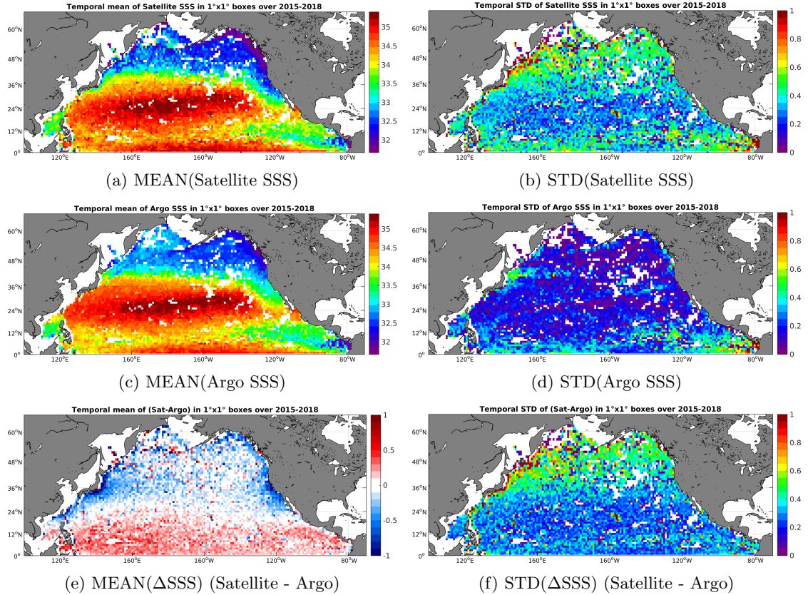
Figure 6: Temporal mean (left) and STD (right) of SSS from SMAP-L3-RSS-V2-8DAY-RUNNING-40KM (top), Argo (middle), and of \Delta SSS (Satellite - Argo). Only match-up pairs are used to generate these maps.
