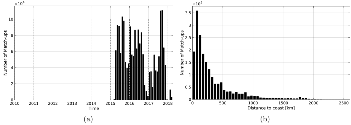
Figure 1: Number of match-ups between TSG-SAMOS and SMAP-L3-RSS-V2-8DAY-RUNNING-70KM SSS as a function of time (a) and as function of the distance to coast (b) over the North Pacific Ocean Pi-MEP region and for the full satellite product period.
