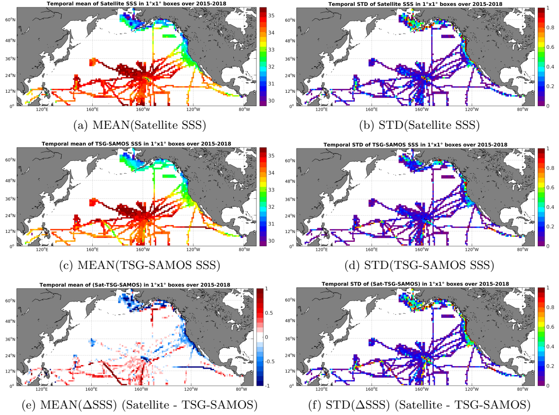
Figure 6: Temporal mean (left) and STD (right) of SSS from SMAP-L3-RSS-V2-8DAY-RUNNING-70KM (top), TSG-SAMOS (middle), and of \Delta SSS (Satellite - TSG-SAMOS). Only match-up pairs are used to generate these maps.
