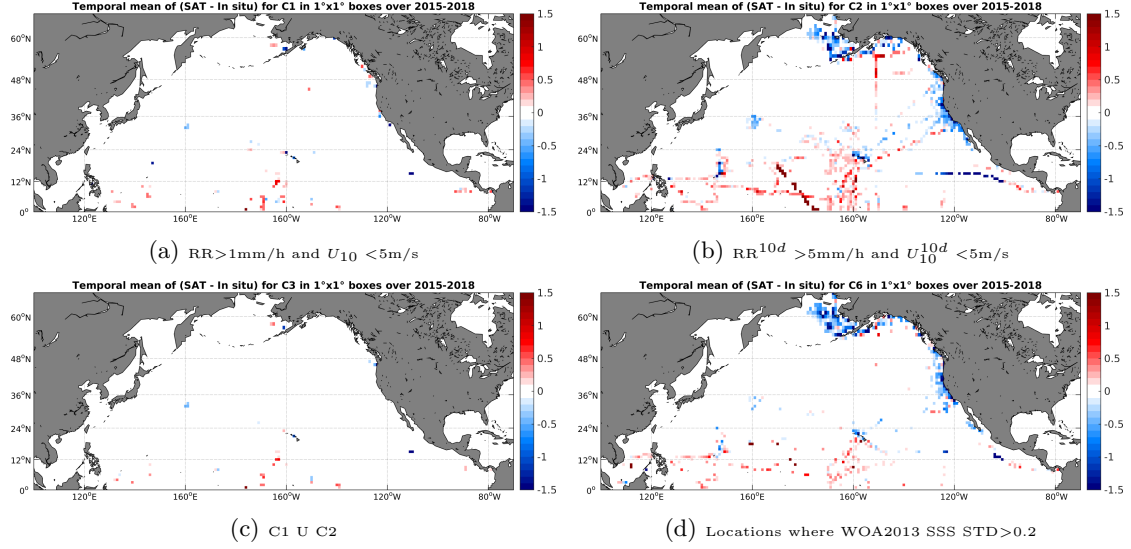
Figure 12: Temporal mean gridded over spatial boxes of size 1^\circ \times 1^\circ of \Delta SSS (SMAP-L3-RSS-V2-8DAY-RUNNING-70KM - TSG-SAMOS) for 4 different subdatasets corresponding to: RR > 1 mm/h and U_{10} < 5 m/s (a), RR^{10d} > 5 mm/h and U_{10}^{10d} < 5 m/s (b), C1 U C2 (c), Locations where WOA2013 SSS STD > 0.2 (d).
