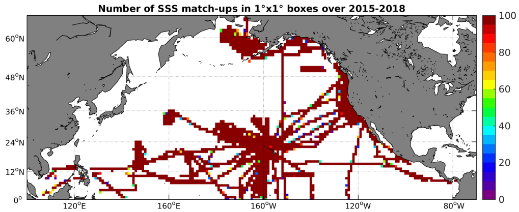
Figure 4: Number of SSS match-ups between TSG-SAMOS SSS and the SMAP-L3-RSS-V2-8DAY-RUNNING-70KM SSS product for the North Pacific Ocean Pi-MEP region over 1^\circ \times 1^\circ boxes and for the full satellite product period.
