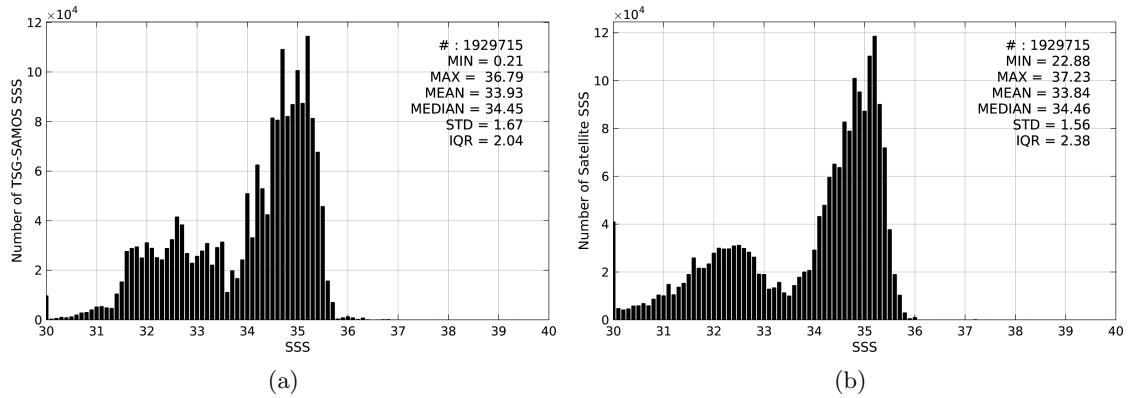
Figure 2: Histograms of SSS from TSG-SAMOS (a) and SMAP-L3-RSS-V2-8DAY-RUNNING-70KM (b) considering all match-up pairs per bins of 0.1 over the North Pacific Ocean Pi-MEP region and for the full satellite product period.
