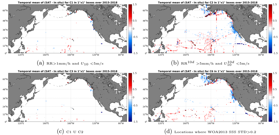
Figure 12: Temporal mean gridded over spatial boxes of size 1^\circ \times 1^\circ of \Delta SSS (SMAP-L3-RSS-V2-MONTHLY-0.25DEG-40KM - TSG-SAMOS) for 4 different subdatasets corresponding to: RR > 1\text{mm/h} and U_{10} < 5\text{m/s} (a), RR^{10d} > 5\text{mm/h} and U_{10}^{10d} < 5\text{m/s} (b), C1 \cup C2 (c), Locations where WOA2013 SSS STD > 0.2 (d).
