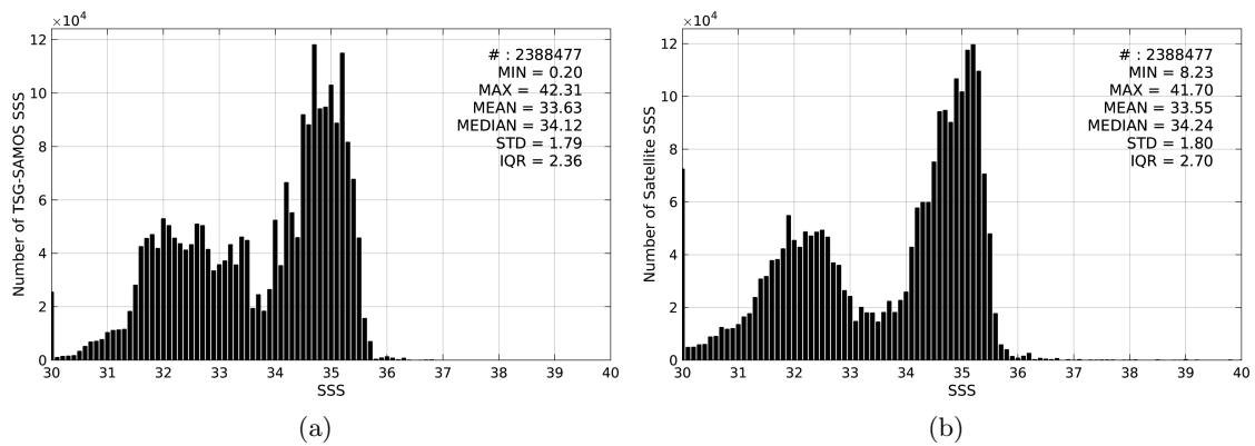
Figure 2: Histograms of SSS from TSG-SAMOS (a) and SMAP-L3-RSS-V2-MONTHLY-0.25DEG-40KM (b) considering all match-up pairs per bins of 0.1 over the North Pacific Ocean Pi-MEP region and for the full satellite product period.
