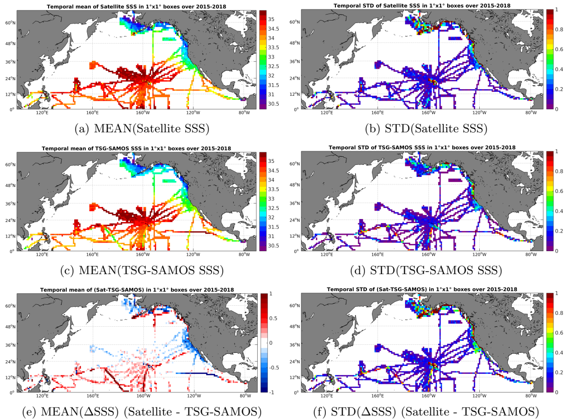
Figure 6: Temporal mean (left) and STD (right) of SSS from SMAP-L3-RSS-V2-MONTHLY-0.25DEG-40KM (top), TSG-SAMOS (middle), and of \Delta SSS (Satellite - TSG-SAMOS). Only match-up pairs are used to generate these maps.
