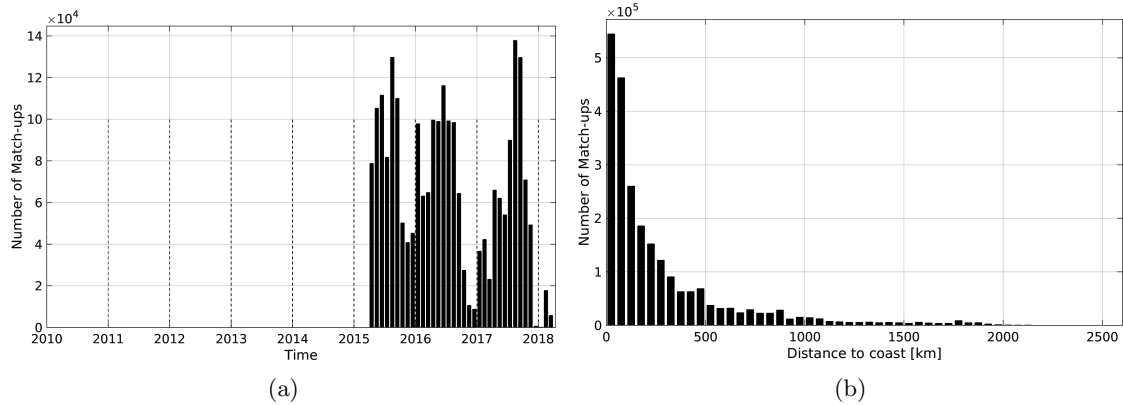
Figure 1: Number of match-ups between TSG-SAMOS and SMAP-L3-RSS-V2-MONTHLY-0.25DEG-40KM SSS as a function of time (a) and as function of the distance to coast (b) over the North Pacific Ocean Pi-MEP region and for the full satellite product period.
