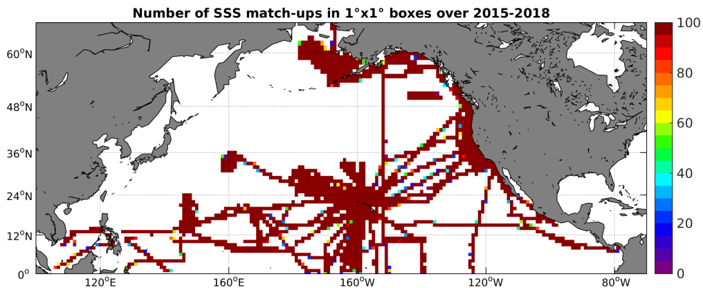
Figure 4: Number of SSS match-ups between TSG-SAMOS SSS and the SMAP-L3-RSS-V2-MONTHLY-0.25DEG-40KM SSS product for the North Pacific Ocean Pi-MEP region over 1^\circ \times 1^\circ boxes and for the full satellite product period.
