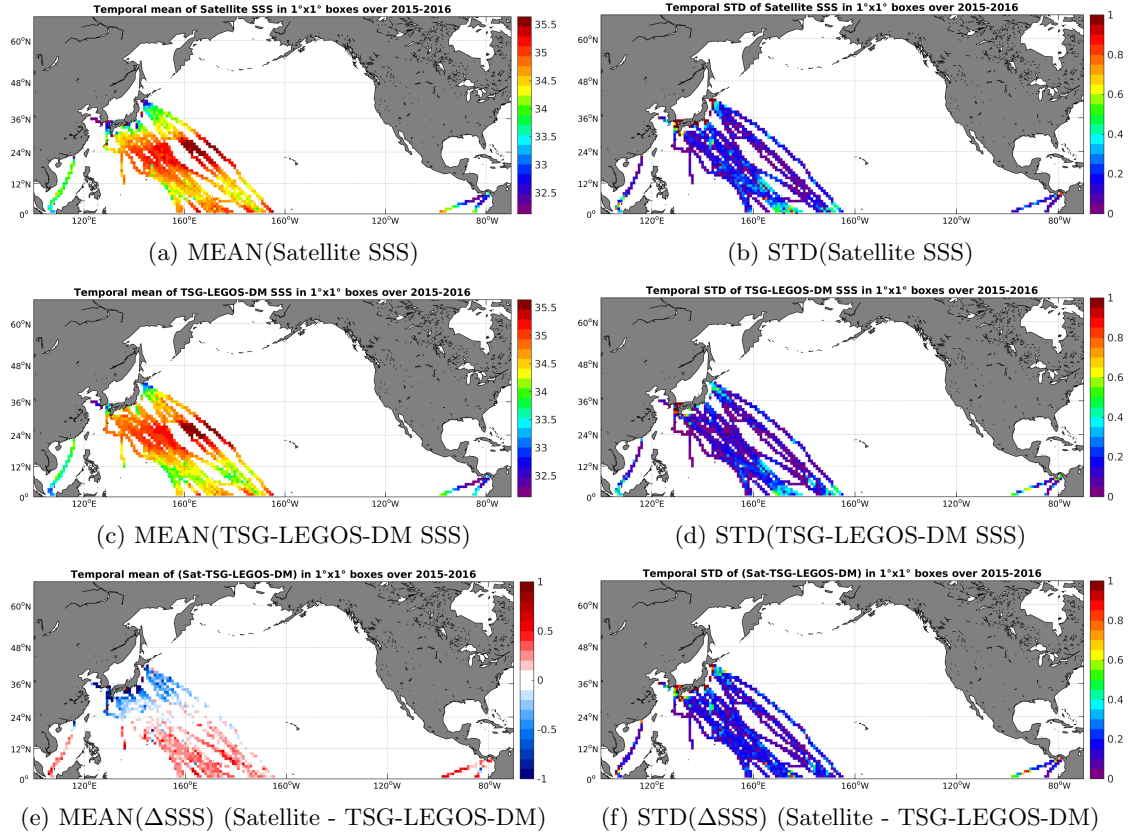
Figure 6: Temporal mean (left) and STD (right) of SSS from SMAP-L3-RSS-V2-MONTHLY-0.25DEG-40KM (top), TSG-LEGOS-DM (middle), and of \Delta SSS (Satellite - TSG-LEGOS-DM). Only match-up pairs are used to generate these maps.
