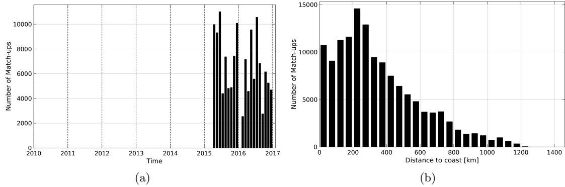
Figure 1: Number of match-ups between TSG-LEGOS-DM and SMAP-L3-RSS-V2-MONTHLY-0.25DEG-40KM SSS as a function of time (a) and as function of the distance to coast (b) over the North Pacific Ocean Pi-MEP region and for the full satellite product period.
