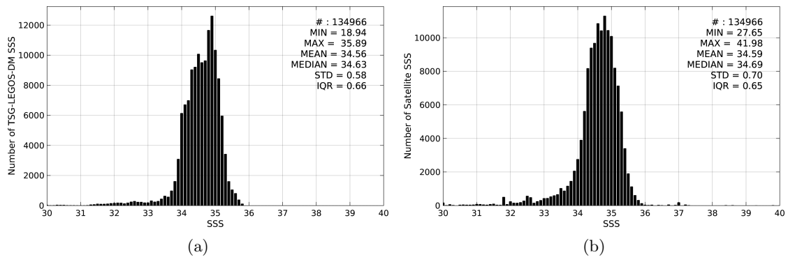
Figure 2: Histograms of SSS from TSG-LEGOS-DM (a) and SMAP-L3-RSS-V2-MONTHLY-0.25DEG-40KM (b) considering all match-up pairs per bins of 0.1 over the North Pacific Ocean Pi-MEP region and for the full satellite product period.
