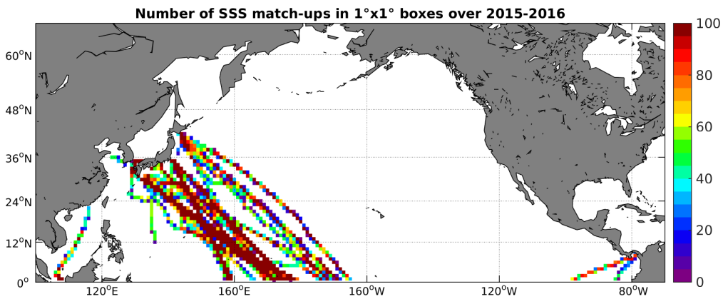
Figure 4: Number of SSS match-ups between TSG-LEGOS-DM SSS and the SMAP-L3-RSS-V2-MONTHLY-0.25DEG-40KM SSS product for the North Pacific Ocean Pi-MEP region over 1^\circ \times 1^\circ boxes and for the full satellite product period.
