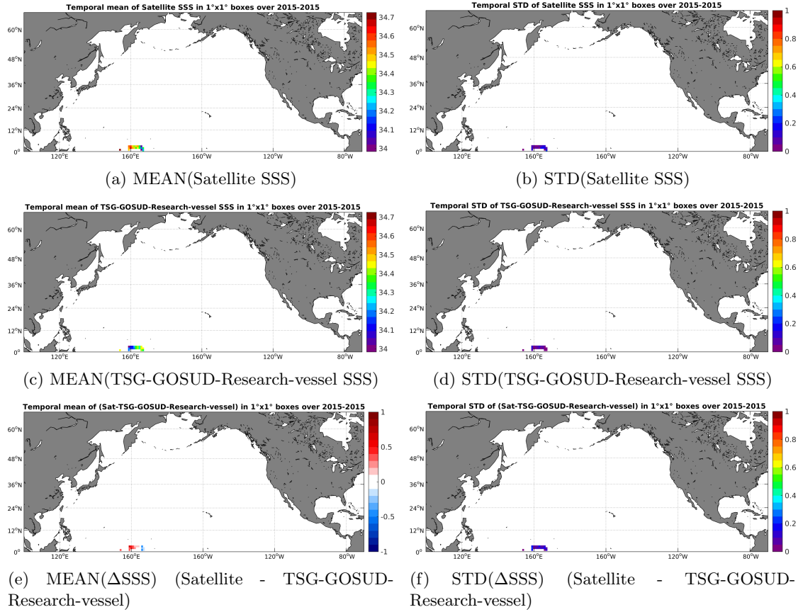
Figure 6: Temporal mean (left) and STD (right) of SSS from SMAP-L3-RSS-V2-MONTHLY-0.25DEG-40KM (top), TSG-GOSUD-Research-vessel (middle), and of \Delta SSS (Satellite - TSG-GOSUD-Research-vessel). Only match-up pairs are used to generate these maps.
