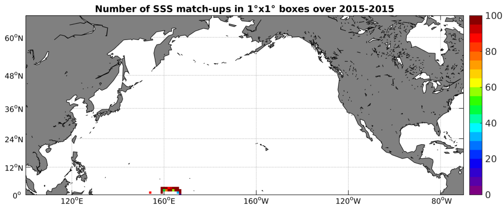
Figure 4: Number of SSS match-ups between TSG-GOSUD-Research-vessel SSS and the SMAP-L3-RSS-V2-MONTHLY-0.25DEG-40KM SSS product for the North Pacific Ocean Pi-MEP region over 1^\circ \times 1^\circ boxes and for the full satellite product period.
