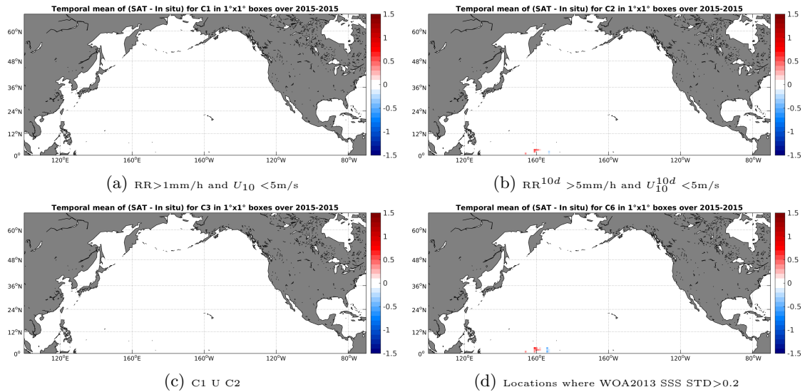
Figure 12: Temporal mean gridded over spatial boxes of size 1^\circ \times 1^\circ of \Delta SSS (SMAP-L3-RSS-V2-MONTHLY-0.25DEG-40KM - TSG-GOSUD-Research-vessel) for 4 different subdatasets corresponding to:RR>1mm/h and U_{10} < 5m/s (a), RR^{10d} > 5mm/h and U_{10}^{10d} < 5m/s (b), C1 U C2 (c),Locations where WOA2013 SSS STD>0.2 (d).
