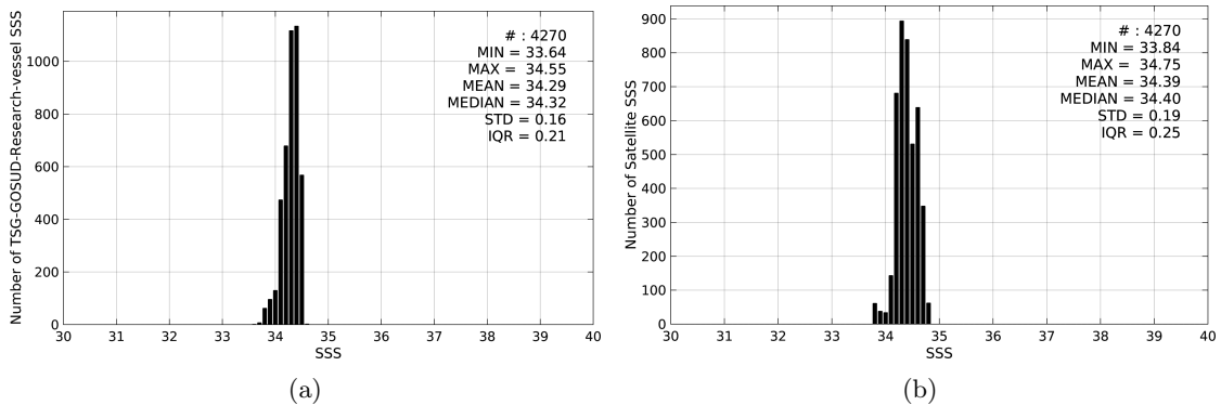
Figure 2: Histograms of SSS from TSG-GOSUD-Research-vessel (a) and SMAP-L3-RSS-V2-MONTHLY-0.25DEG-40KM (b) considering all match-up pairs per bins of 0.1 over the North Pacific Ocean Pi-MEP region and for the full satellite product period.
