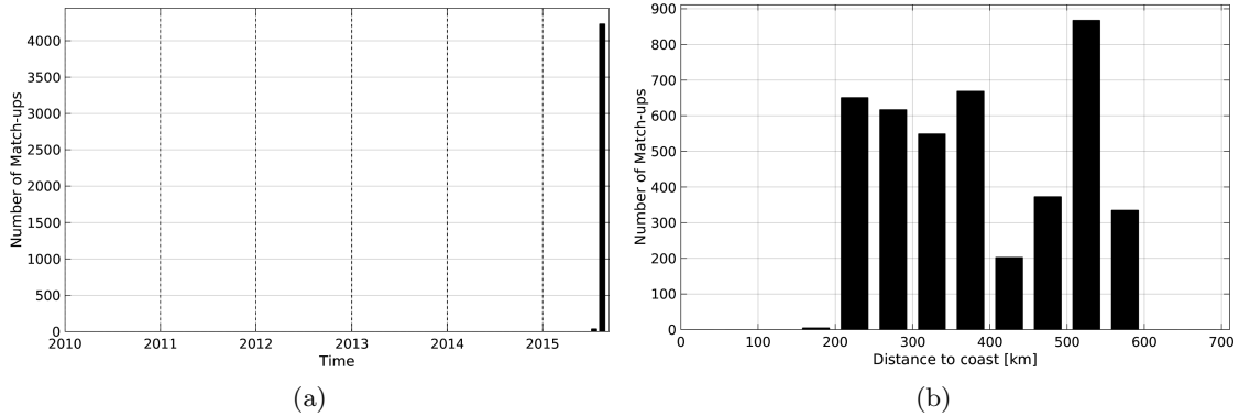
Figure 1: Number of match-ups between TSG-GOSUD-Research-vessel and SMAP-L3-RSS-V2-MONTHLY-0.25DEG-40KM SSS as a function of time (a) and as function of the distance to coast (b) over the North Pacific Ocean Pi-MEP region and for the full satellite product period.
