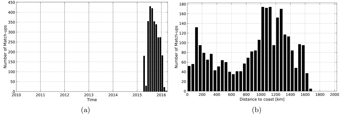
Figure 1: Number of match-ups between Sea mammals and SMAP-L3-RSS-V2-MONTHLY-0.25DEG-40KM SSS as a function of time (a) and as function of the distance to coast (b) over the North Pacific Ocean Pi-MEP region and for the full satellite product period.
