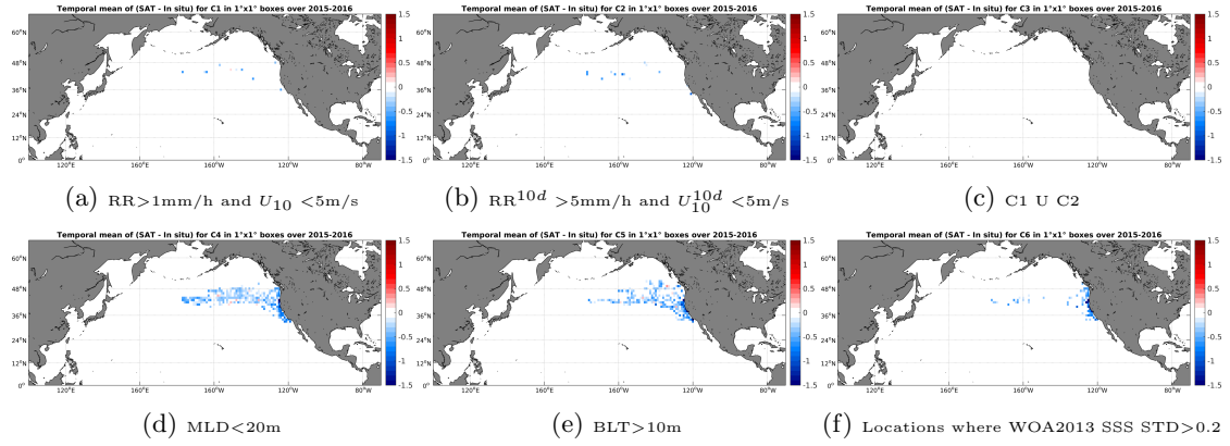
Figure 12: Temporal mean gridded over spatial boxes of size 1^\circ \times 1^\circ of \Delta SSS (SMAP-L3-RSS-V2-MONTHLY-0.25DEG-40KM - Sea mammals) for 6 different subdatasets corresponding to: RR > 1\text{mm/h} and U_{10} < 5\text{m/s} (a), RR^{10d} > 5\text{mm/h} and U_{10}^{10d} < 5\text{m/s} (b), C1 U C2 (c), MLD < 20\text{m} (d), BLT > 10\text{m} (e), Locations where WOA2013 SSS STD > 0.2 (f).
