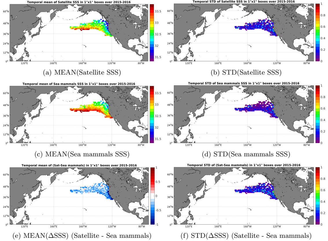
Figure 6: Temporal mean (left) and STD (right) of SSS from SMAP-L3-RSS-V2-MONTHLY-0.25DEG-40KM (top), Sea mammals (middle), and of \Delta SSS (Satellite - Sea mammals). Only match-up pairs are used to generate these maps.
