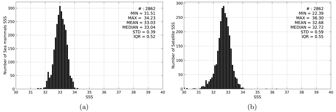
Figure 2: Histograms of SSS from Sea mammals (a) and SMAP-L3-RSS-V2-MONTHLY-0.25DEG-40KM (b) considering all match-up pairs per bins of 0.1 over the North Pacific Ocean Pi-MEP region and for the full satellite product period.
