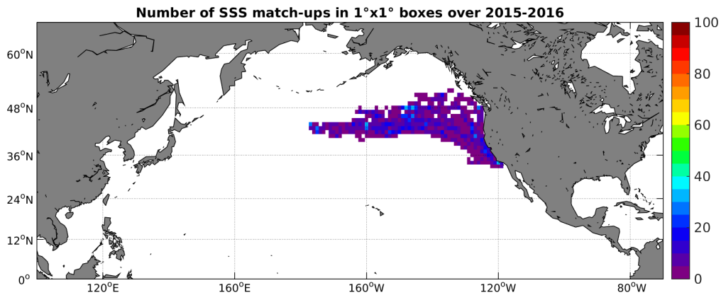
Figure 4: Number of SSS match-ups between Sea mammals SSS and the SMAP-L3-RSS-V2-MONTHLY-0.25DEG-40KM SSS product for the North Pacific Ocean Pi-MEP region over 1^\circ \times 1^\circ boxes and for the full satellite product period.
