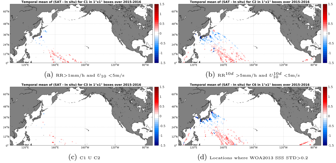
Figure 12: Temporal mean gridded over spatial boxes of size 1^\circ \times 1^\circ of \Delta SSS (SMAP-L3-RSS-V2-MONTHLY-70KM - TSG-LEGOS-DM) for 4 different subdatasets corresponding to: RR > 1 mm/h and U_{10} < 5 m/s (a), RR^{10d} > 5 mm/h and U_{10}^{10d} < 5 m/s (b), C1 U C2 (c), Locations where WOA2013 SSS STD > 0.2 (d).
