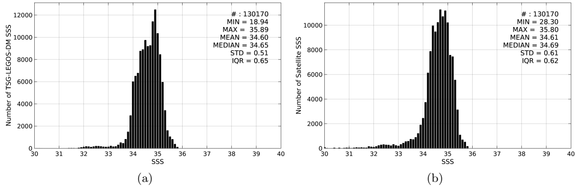
Figure 2: Histograms of SSS from TSG-LEGOS-DM (a) and SMAP-L3-RSS-V2-MONTHLY-70KM (b) considering all match-up pairs per bins of 0.1 over the North Pacific Ocean Pi-MEP region and for the full satellite product period.
