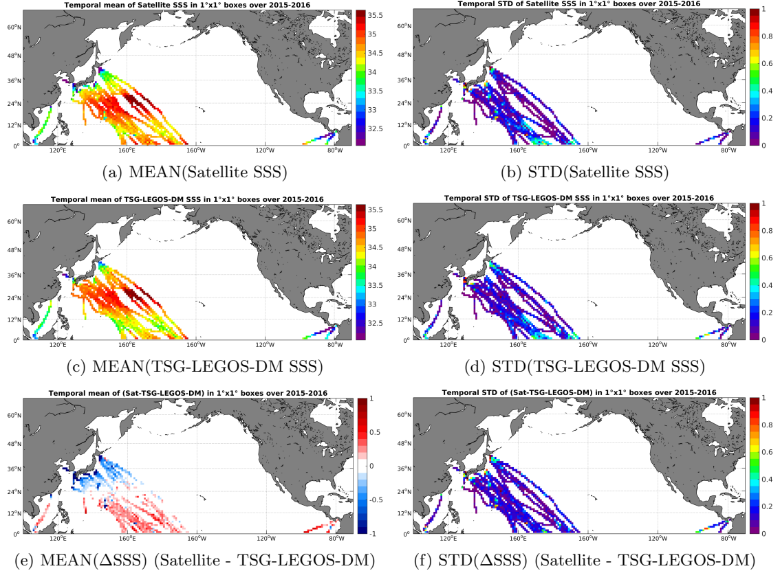
Figure 6: Temporal mean (left) and STD (right) of SSS from SMAP-L3-RSS-V2-MONTHLY-70KM (top), TSG-LEGOS-DM (middle), and of \Delta SSS (Satellite - TSG-LEGOS-DM). Only match-up pairs are used to generate these maps.
