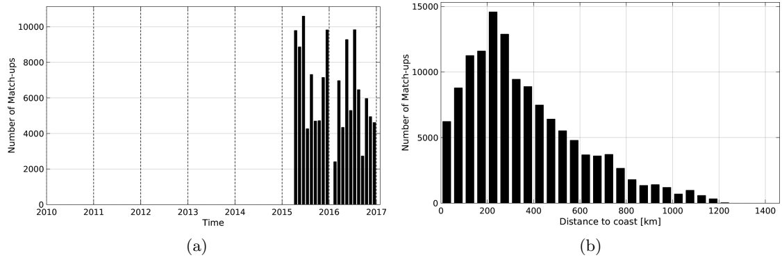
Figure 1: Number of match-ups between TSG-LEGOS-DM and SMAP-L3-RSS-V2-MONTHLY-70KM SSS as a function of time (a) and as function of the distance to coast (b) over the North Pacific Ocean Pi-MEP region and for the full satellite product period.
