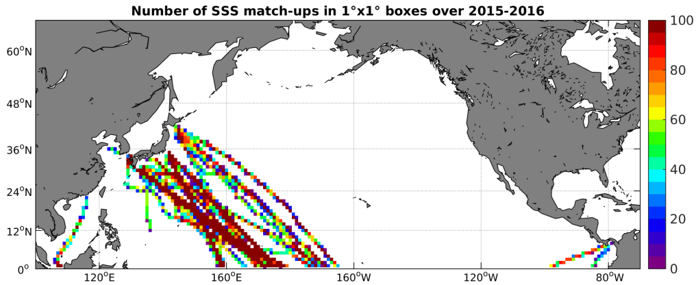
Figure 4: Number of SSS match-ups between TSG-LEGOS-DM SSS and the SMAP-L3-RSS-V2-MONTHLY-70KM SSS product for the North Pacific Ocean Pi-MEP region over 1^\circ \times 1^\circ boxes and for the full satellite product period.
