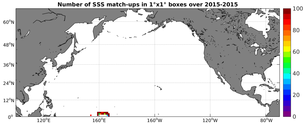
Figure 4: Number of SSS match-ups between TSG-GOSUD-Research-vessel SSS and the SMAP-L3-RSS-V2-MONTHLY-70KM SSS product for the North Pacific Ocean Pi-MEP region over 1^\circ \times 1^\circ boxes and for the full satellite product period.
