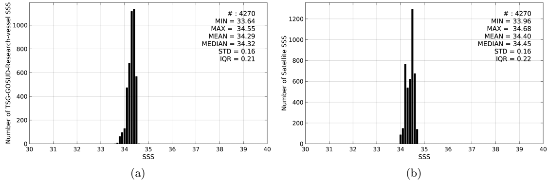
Figure 2: Histograms of SSS from TSG-GOSUD-Research-vessel (a) and SMAP-L3-RSS-V2-MONTHLY-70KM (b) considering all match-up pairs per bins of 0.1 over the North Pacific Ocean Pi-MEP region and for the full satellite product period.
