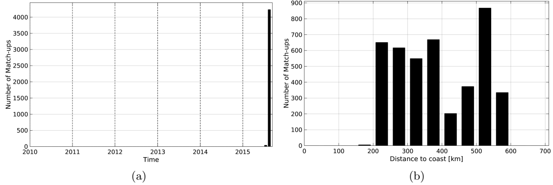
Figure 1: Number of match-ups between TSG-GOSUD-Research-vessel and SMAP-L3-RSS-V2-MONTHLY-70KM SSS as a function of time (a) and as function of the distance to coast (b) over the North Pacific Ocean Pi-MEP region and for the full satellite product period.
