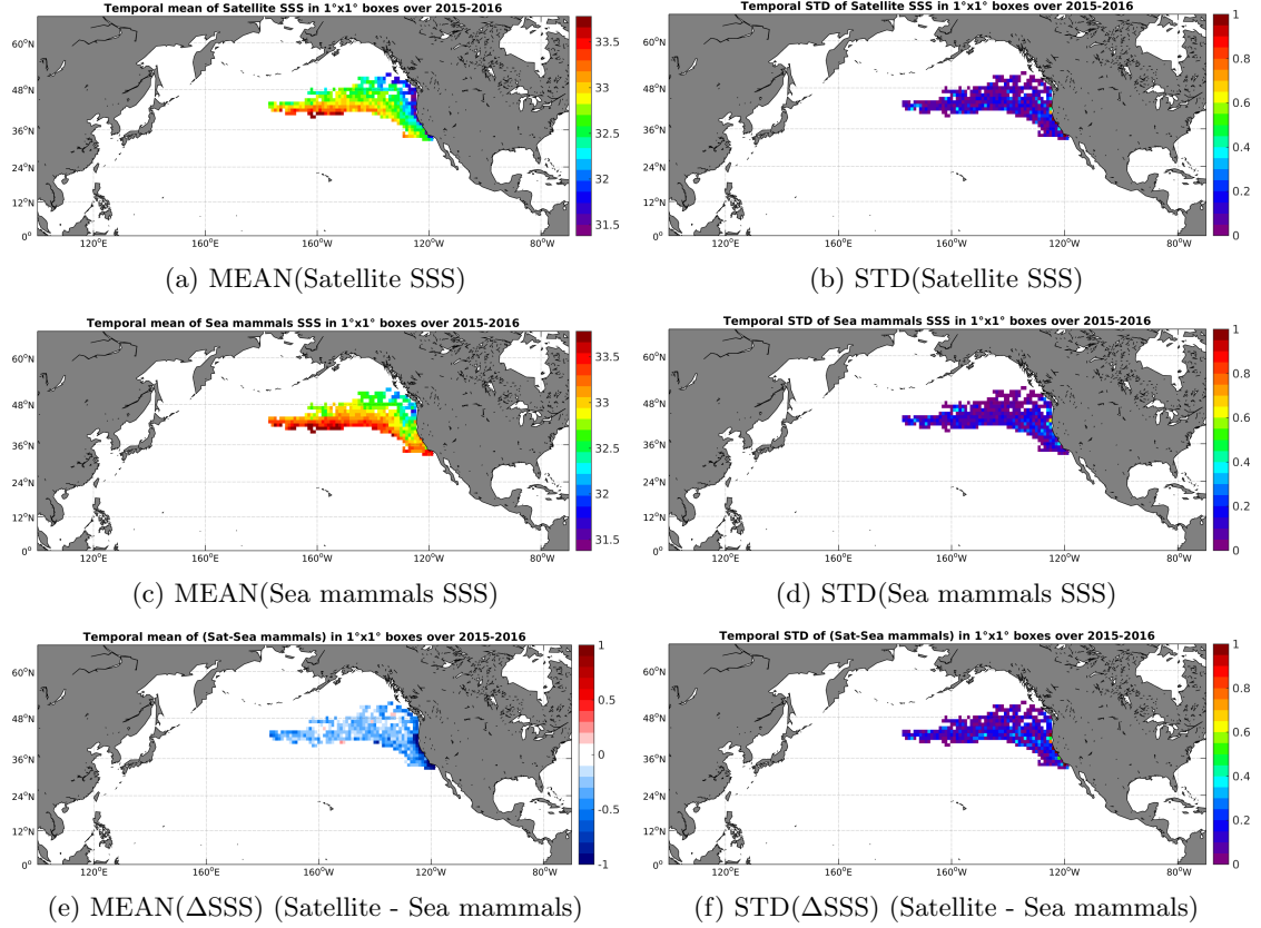
Figure 6: Temporal mean (left) and STD (right) of SSS from SMAP-L3-RSS-V2-MONTHLY-70KM (top), Sea mammals (middle), and of \Delta SSS (Satellite - Sea mammals). Only match-up pairs are used to generate these maps.
