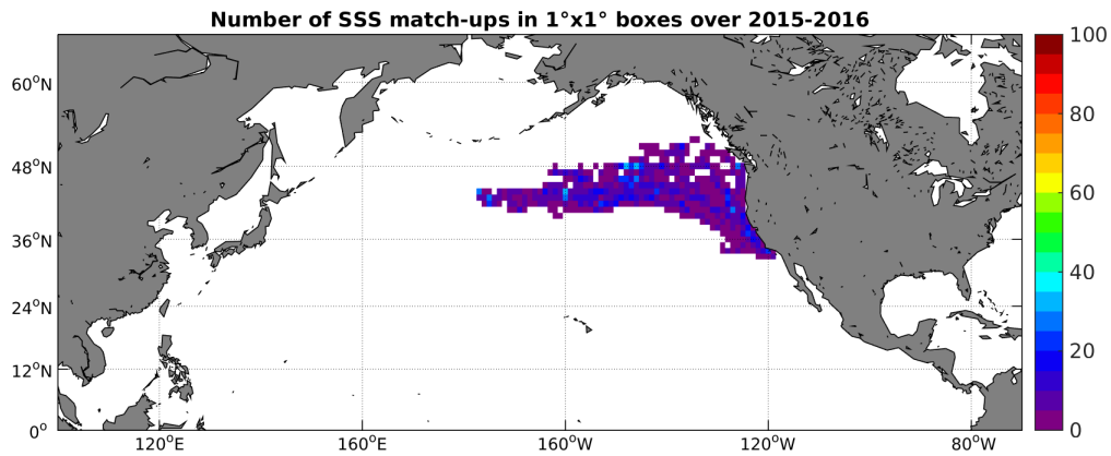
Figure 4: Number of SSS match-ups between Sea mammals SSS and the SMAP-L3-RSS-V2-MONTHLY-70KM SSS product for the North Pacific Ocean Pi-MEP region over 1^\circ \times 1^\circ boxes and for the full satellite product period.
