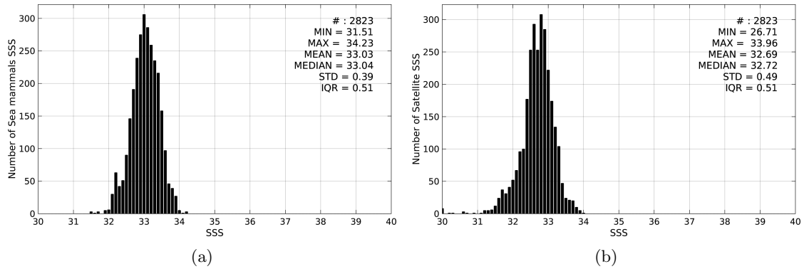
Figure 2: Histograms of SSS from Sea mammals (a) and SMAP-L3-RSS-V2-MONTHLY-70KM (b) considering all match-up pairs per bins of 0.1 over the North Pacific Ocean Pi-MEP region and for the full satellite product period.
