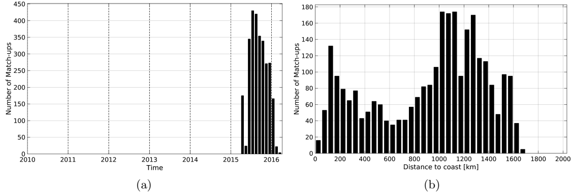
Figure 1: Number of match-ups between Sea mammals and SMAP-L3-RSS-V2-MONTHLY-70KM SSS as a function of time (a) and as function of the distance to coast (b) over the North Pacific Ocean Pi-MEP region and for the full satellite product period.
