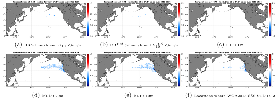
Figure 12: Temporal mean gridded over spatial boxes of size 1^\circ \times 1^\circ of \Delta SSS (SMAP-L3-RSS-V2-MONTHLY-70KM - Sea mammals) for 6 different subdatasets corresponding to: RR > 1\text{mm/h} and U_{10} < 5\text{m/s} (a), RR^{10d} > 5\text{mm/h} and U_{10}^{10d} < 5\text{m/s} (b), C1 U C2 (c), MLD < 20\text{m} (d), BLT > 10\text{m} (e), Locations where WOA2013 SSS STD > 0.2 (f).
