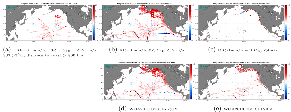
Figure 14: Temporal mean gridded over spatial boxes of size 1^\circ \times 1^\circ of \Delta SSS (SMAP SSS L3 v5.0 - 8-Day running (JPL) - TSG (SAMOS)) for 5 different subdatasets corresponding to: RR=0 mm/h, 3 < U_{10} < 12 m/s, SST > 5°C, distance to coast > 800 km (a), RR=0 mm/h, 3 < U_{10} < 12 m/s (b), RR > 1mm/h and U_{10} < 4 m/s (c), WOA2013 SSS Std < 0.2 (d), WOA2013 SSS Std > 0.2 (e).
